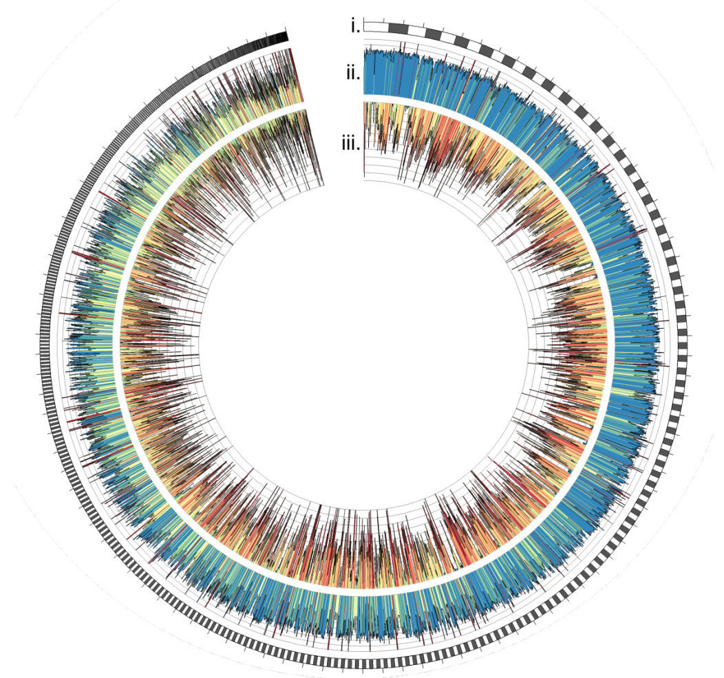
S2 Fig: Redundant primary contig reduction. Circular representations of A) FALCON Unzip Chardonnay assembly and B) the same assembly after curation. Tracks are: length-ordered contigs (i) , read-depth of mapped Illumina paired end reads (ii) and heterozygous SNPs density (iii)
