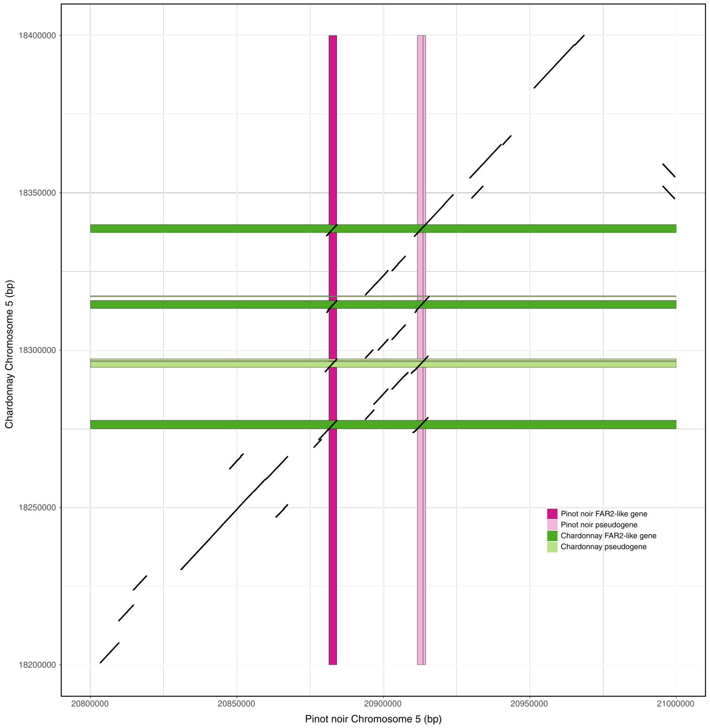
S3 Figure: Gene expansion of Chardonnay Chromosome 5 (primary contigs) region containing FAR2-like genes. Alignments are indicated as black lines (dotplot), the ORFs for FAR2-like genes and pseudogenes are indicated for both Pinot noir and Chardonnay.
