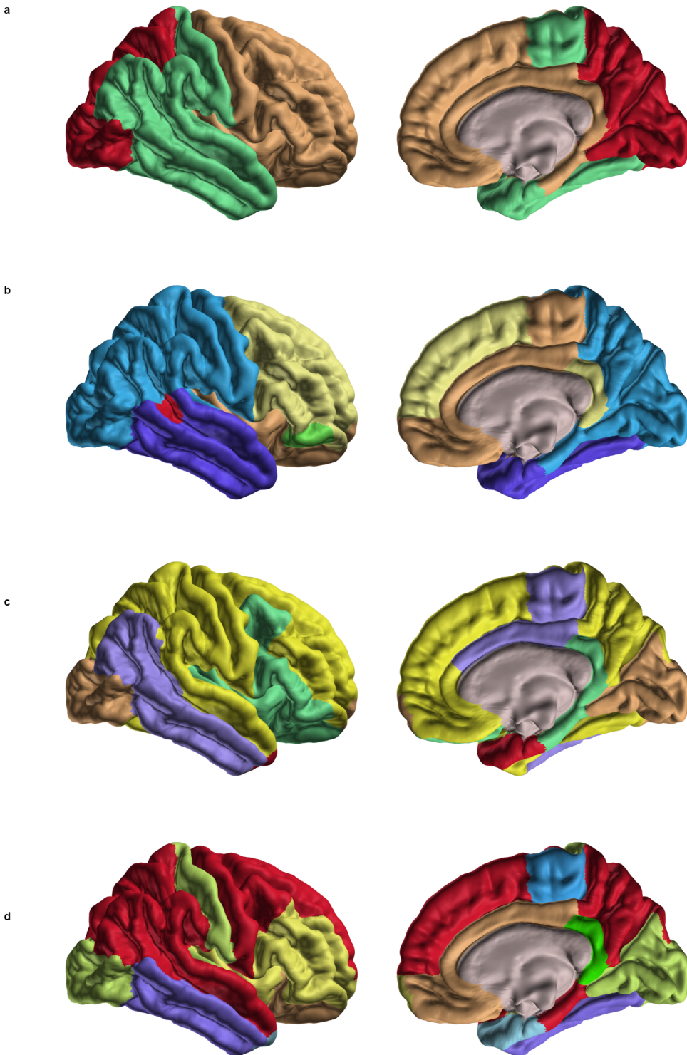
Supplementary Table 3. Clustering of genetic correlations among a) surface area and b) thickness regions after correcting for global measures. Clustering of genetic correlations among c) surface area and d) thickness regions without correcting for global measures. The best-fitting model for surface area with global correction was 3 diagonal components with varying volume and shape, and for thickness was 6 spherical components with equal volume. The best-fitting model for surface area without global correction was 5 spherical components with varying volume, and for thickness was 8 spherical components with equal volume.
