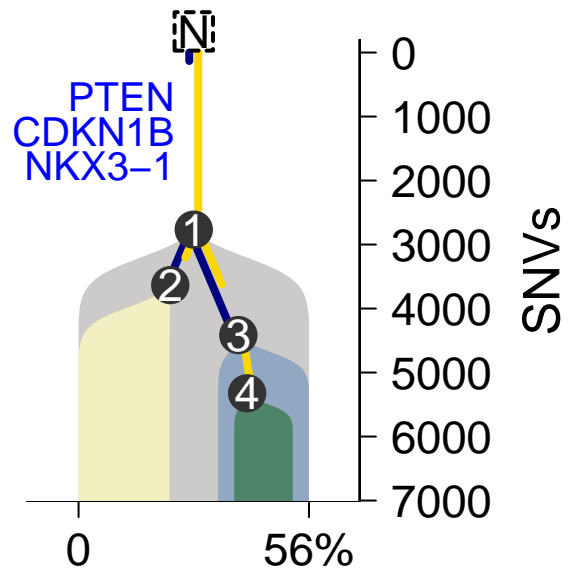
MuTect–TITAN
