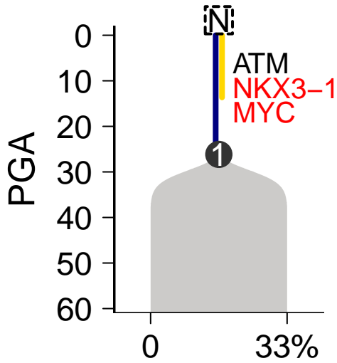
SomaticSniper–Battenberg
