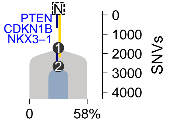
SomaticSniper-TITAN
