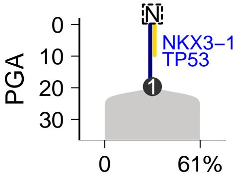
SomaticSniper-Battenberg
