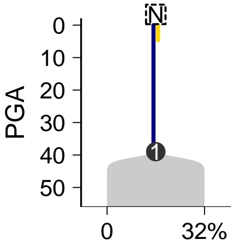
SomaticSniper-Battenberg
