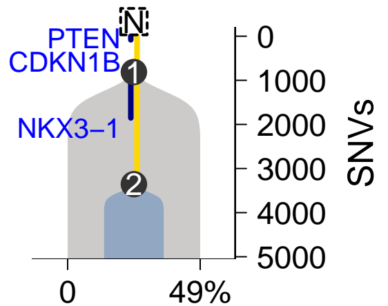
MuTect–TITAN
