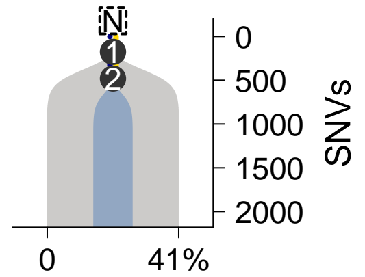
SomaticSniper-TITAN
