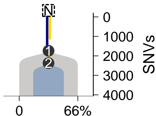
SomaticSniper-TITAN
