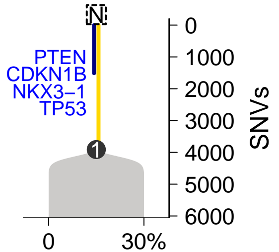
MuTect–TITAN
