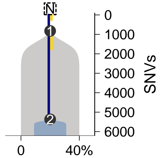
SomaticSniper-TITAN
