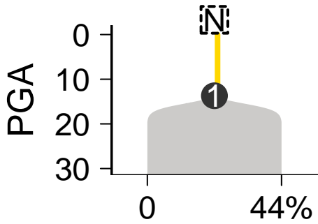
SomaticSniper-Battenberg
