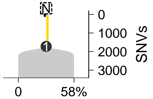
SomaticSniper-TITAN
