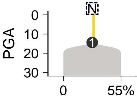
SomaticSniper-Battenberg
