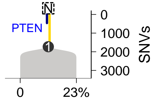
SomaticSniper-TITAN
