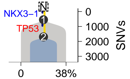
SomaticSniper-TITAN
