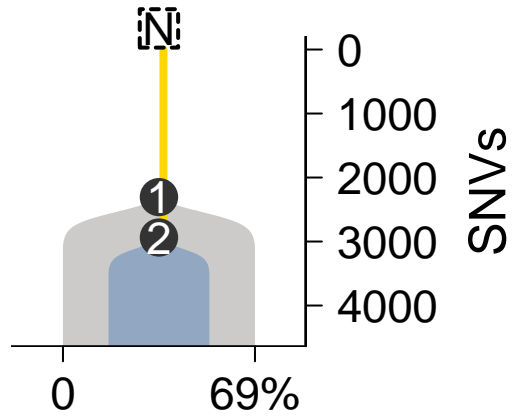
SomaticSniper-TITAN
