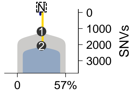
SomaticSniper-TITAN
