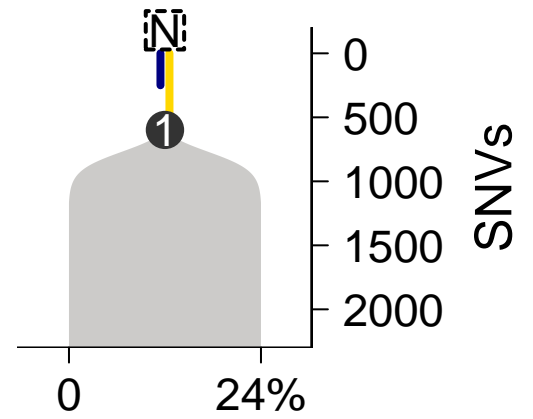
SomaticSniper-TITAN
