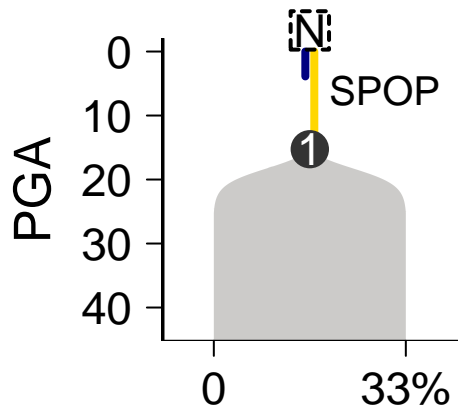
SomaticSniper-Battenberg
