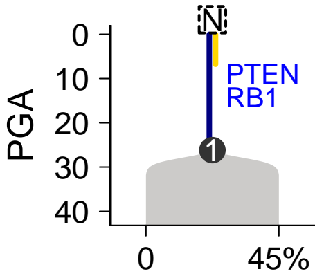
SomaticSniper-Battenberg
