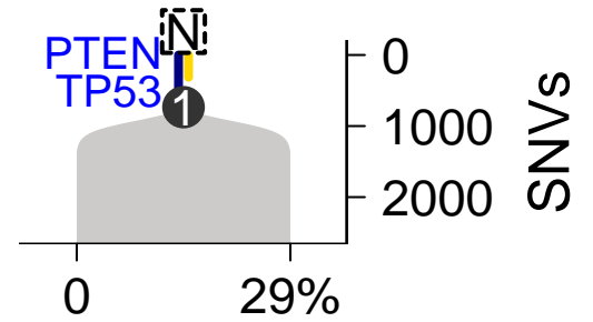
SomaticSniper-TITAN
