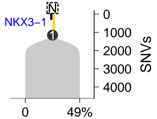
SomaticSniper-TITAN
