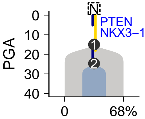
SomaticSniper-Battenberg
