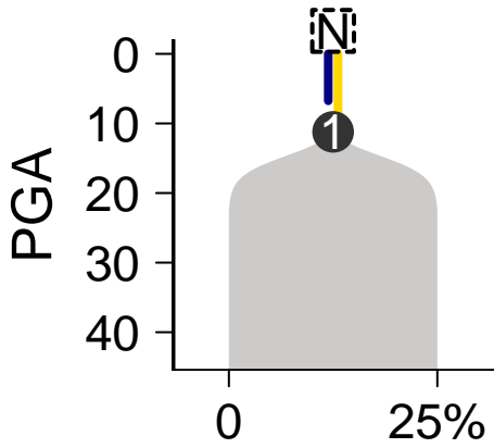
SomaticSniper-Battenberg
