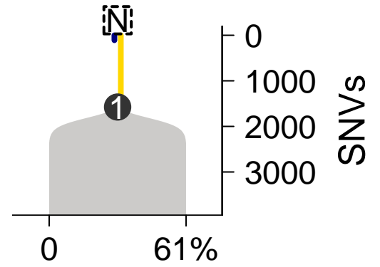
SomaticSniper-TITAN
