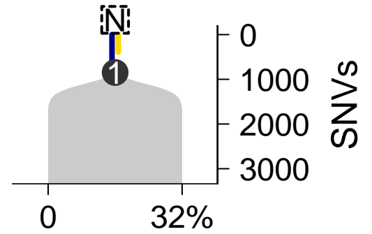
SomaticSniper-TITAN
