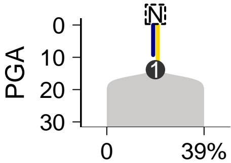
SomaticSniper–Battenberg
