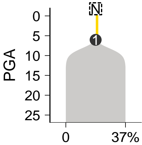
SomaticSniper-Battenberg
