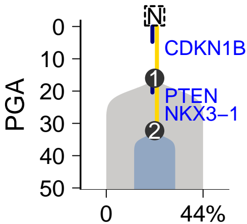
MuTect–Battenberg
