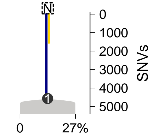
SomaticSniper-TITAN
