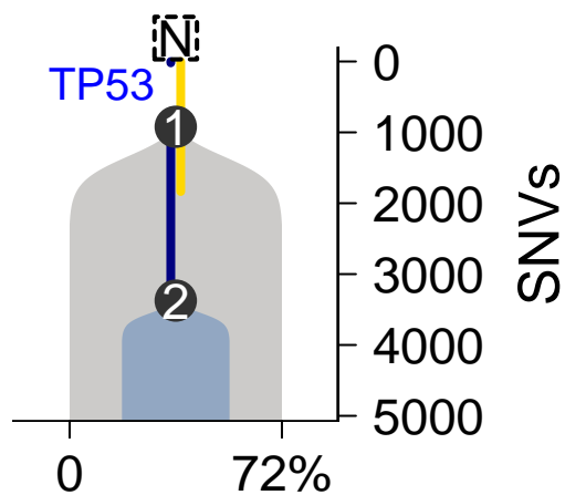
SomaticSniper-TITAN
