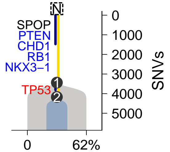
SomaticSniper-TITAN
