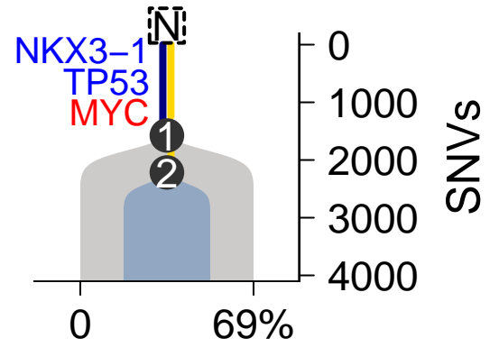
SomaticSniper-TITAN
