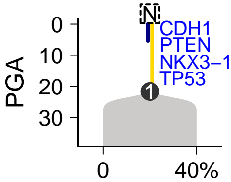
SomaticSniper–Battenberg
