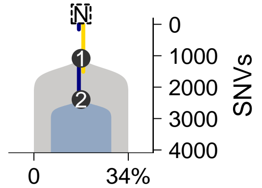
SomaticSniper-TITAN
