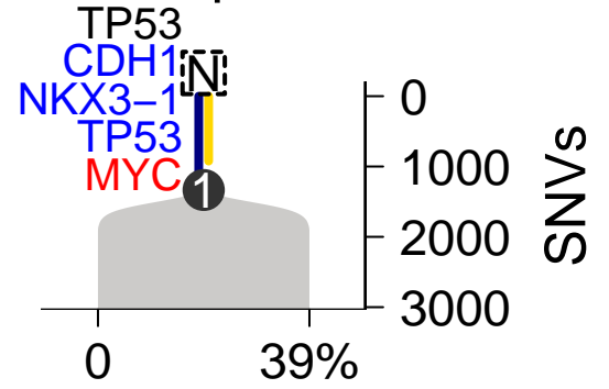
SomaticSniper-TITAN
