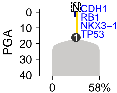
SomaticSniper-Battenberg
