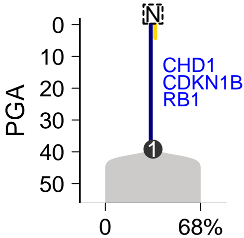
SomaticSniper-Battenberg
