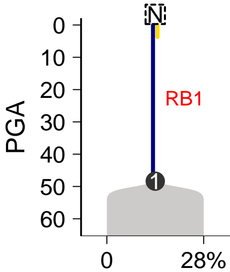
SomaticSniper-Battenberg
