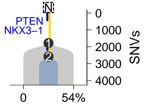
SomaticSniper-TITAN
