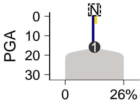
SomaticSniper-Battenberg
