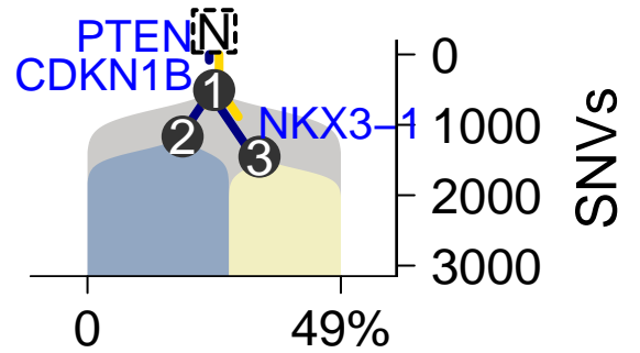
SomaticSniper–TITAN
