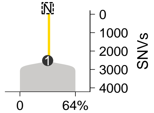
SomaticSniper-TITAN
