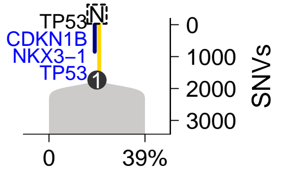
SomaticSniper-TITAN
