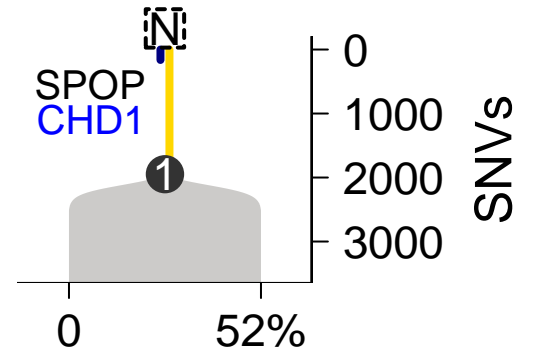
SomaticSniper-TITAN
