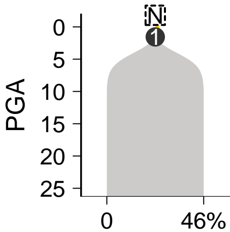
SomaticSniper-Battenberg
