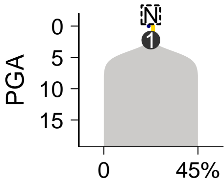
SomaticSniper-Battenberg
