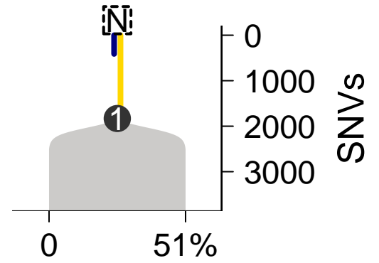
SomaticSniper-TITAN
