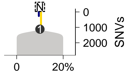
SomaticSniper-TITAN
