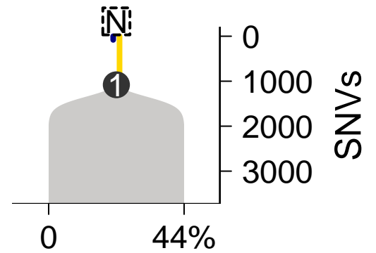
SomaticSniper-TITAN
