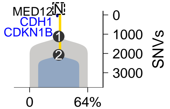
SomaticSniper–TITAN
