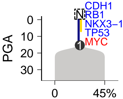
SomaticSniper-Battenberg
