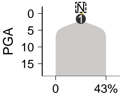
SomaticSniper-Battenberg
