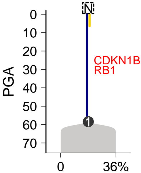
SomaticSniper-Battenberg
