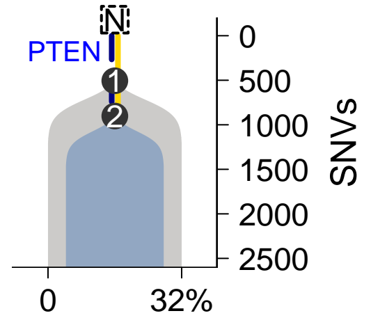
SomaticSniper–TITAN
