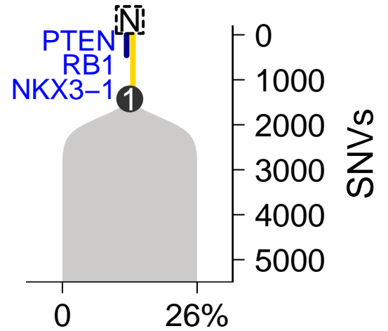
SomaticSniper-TITAN
