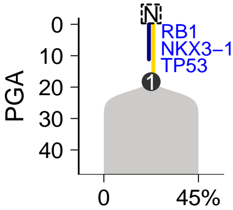
SomaticSniper-Battenberg
