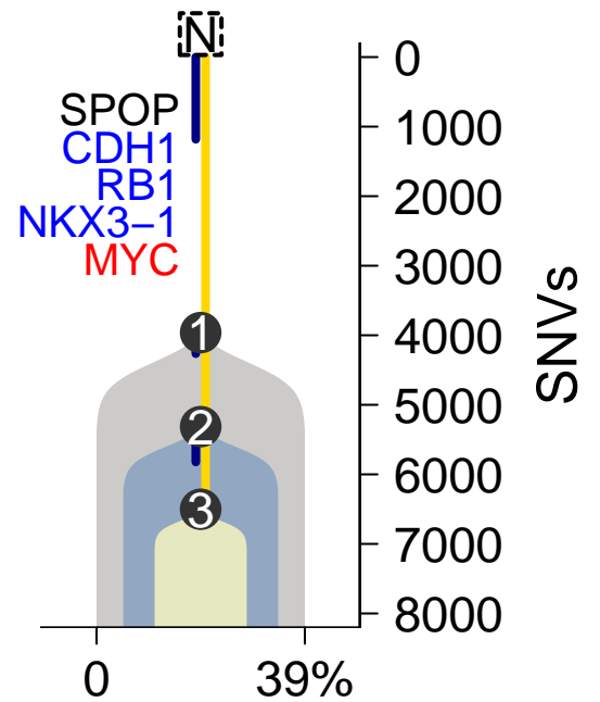
MuTect–TITAN
