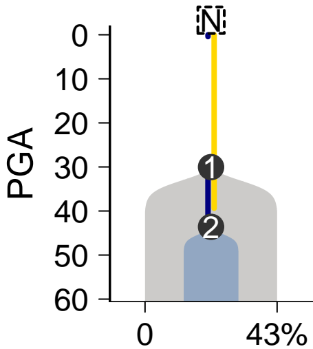
MuTect–Battenberg
