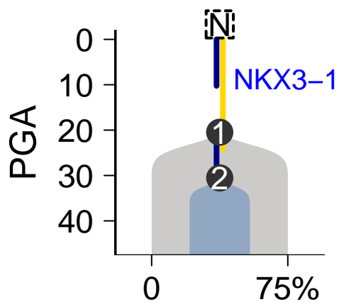
SomaticSniper-Battenberg
