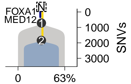
SomaticSniper-TITAN
