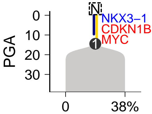
SomaticSniper-Battenberg
