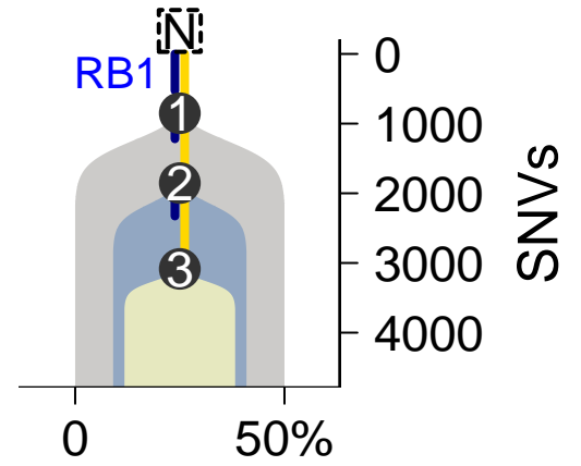
SomaticSniper-TITAN
