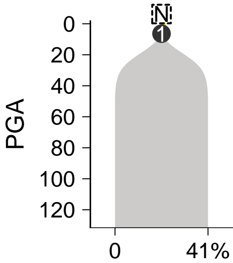
SomaticSniper-Battenberg
