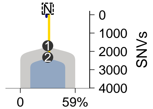
SomaticSniper-TITAN
