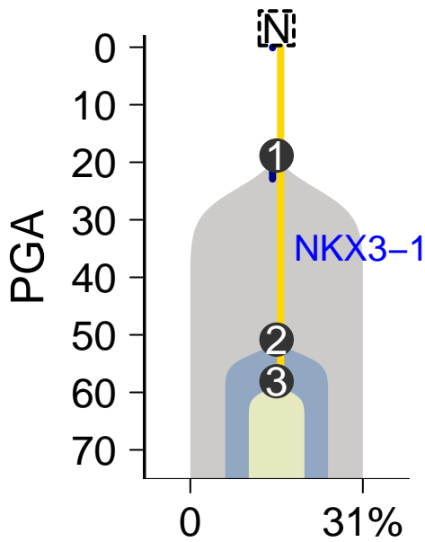
MuTect–Battenberg
