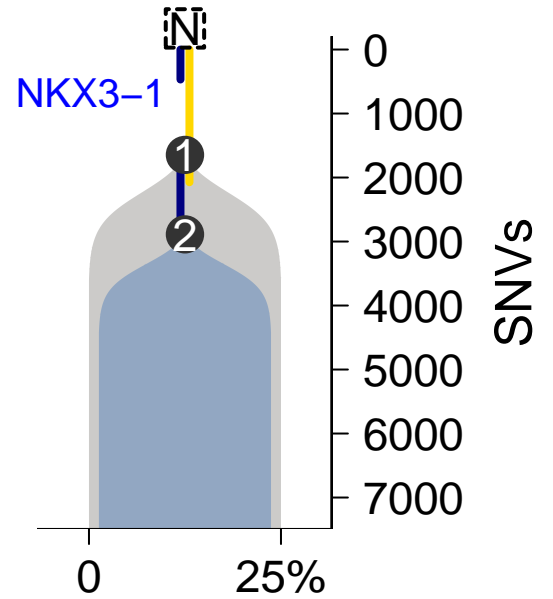
SomaticSniper–TITAN
