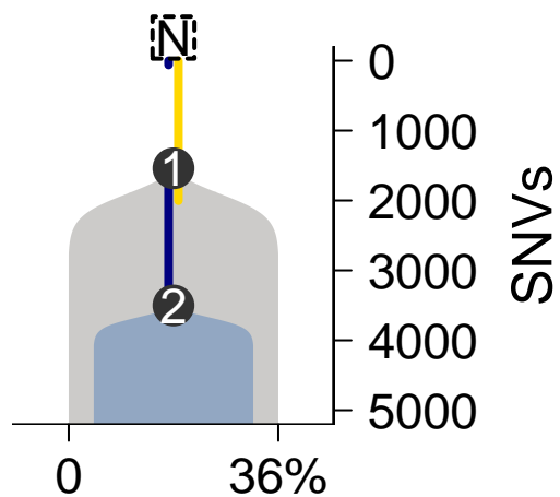
SomaticSniper-TITAN
