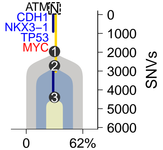
SomaticSniper–TITAN
