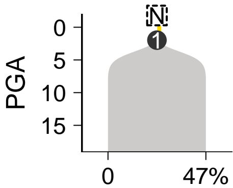
SomaticSniper-Battenberg
