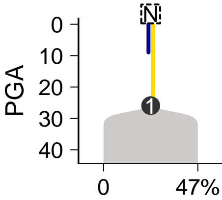
SomaticSniper-Battenberg
