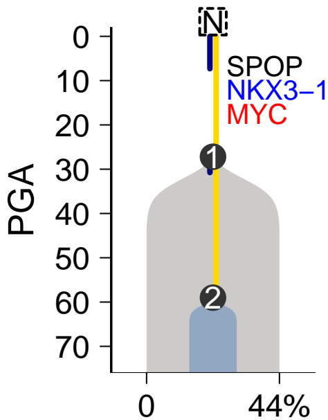
MuTect–Battenberg
