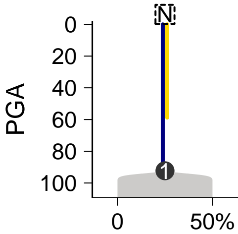
SomaticSniper-Battenberg
