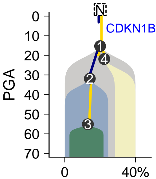
MuTect–Battenberg
