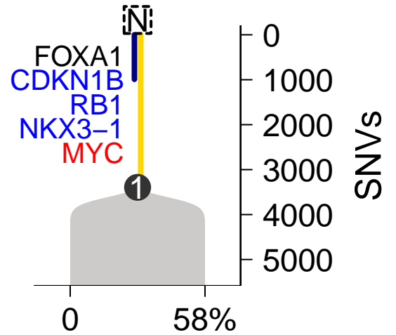
SomaticSniper–TITAN
