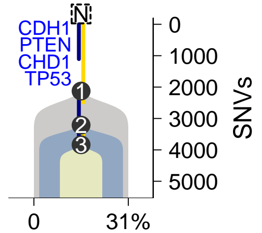
SomaticSniper–TITAN
