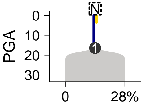
SomaticSniper-Battenberg
