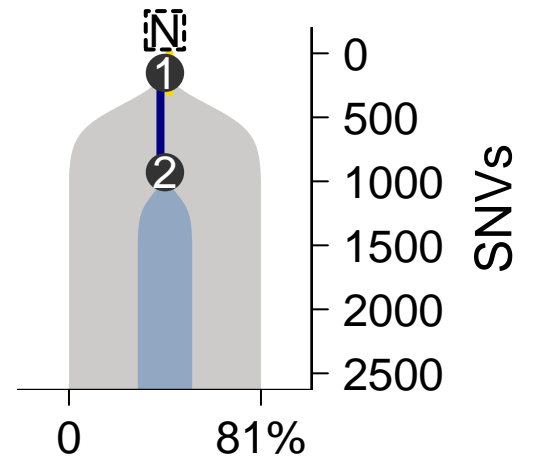
SomaticSniper-TITAN
