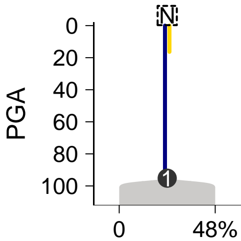
SomaticSniper-Battenberg
