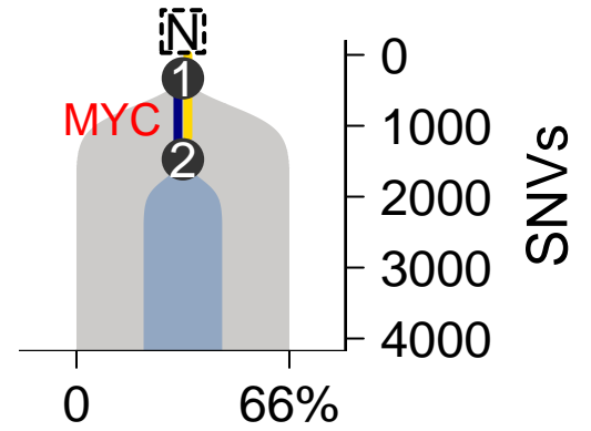
SomaticSniper-TITAN
