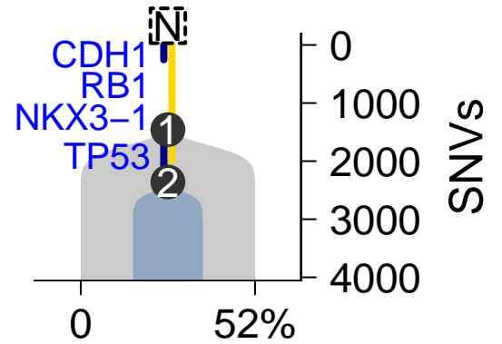
SomaticSniper-TITAN
