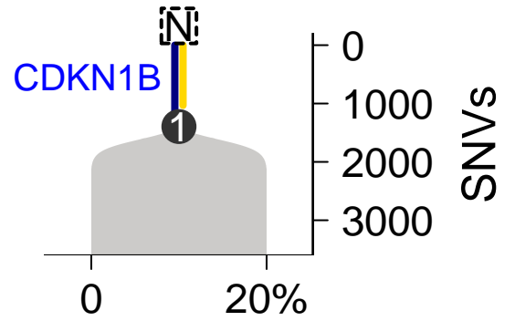
SomaticSniper-TITAN
