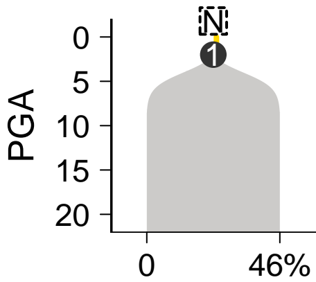
SomaticSniper–Battenberg
