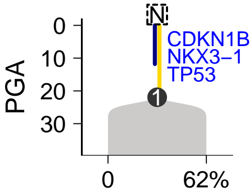
SomaticSniper-Battenberg
