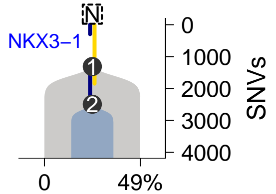
SomaticSniper-TITAN
