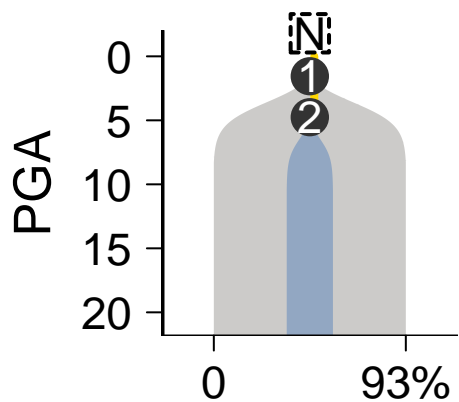
SomaticSniper-Battenberg
