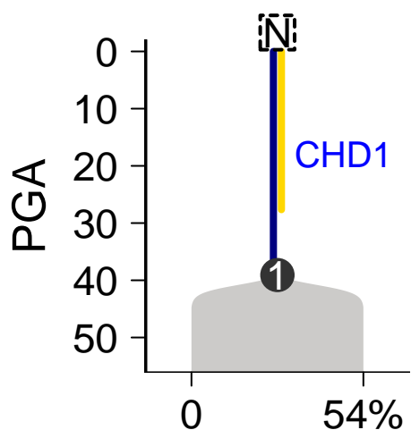
SomaticSniper-Battenberg
