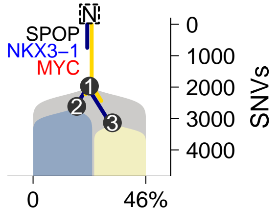
SomaticSniper–TITAN
