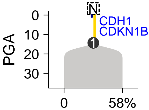
SomaticSniper–Battenberg
