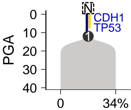
SomaticSniper–Battenberg
