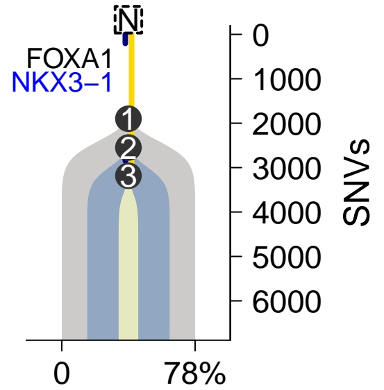
SomaticSniper-TITAN
