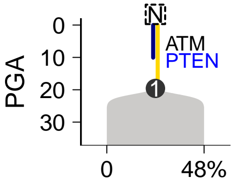
SomaticSniper-Battenberg
