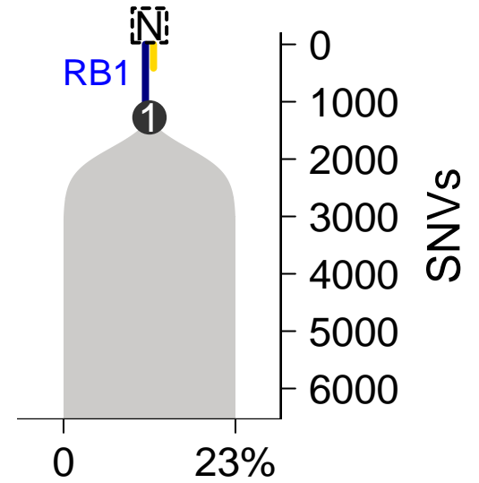
SomaticSniper-TITAN
