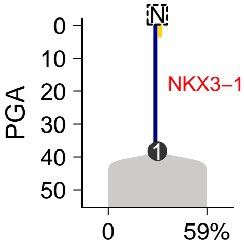
SomaticSniper-Battenberg
