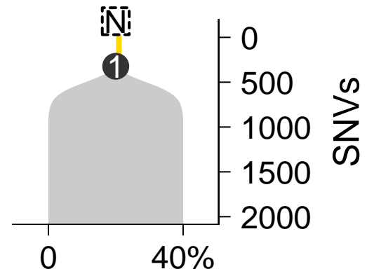
SomaticSniper-TITAN
