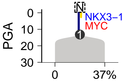
SomaticSniper-Battenberg
