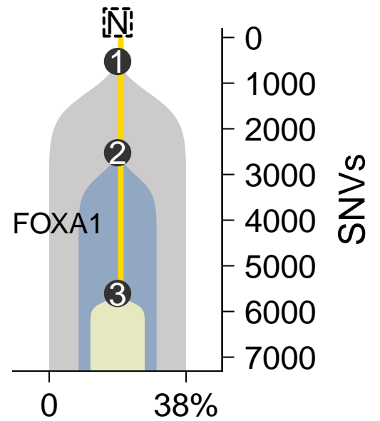
MuTect–TITAN
