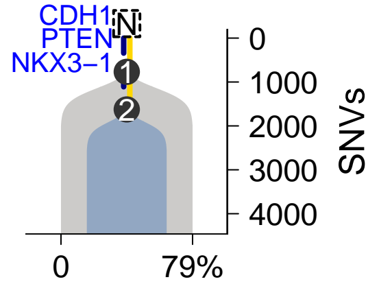
SomaticSniper-TITAN
