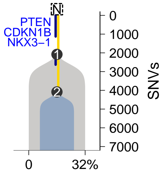
MuTect–TITAN
