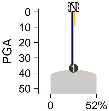
SomaticSniper-Battenberg
