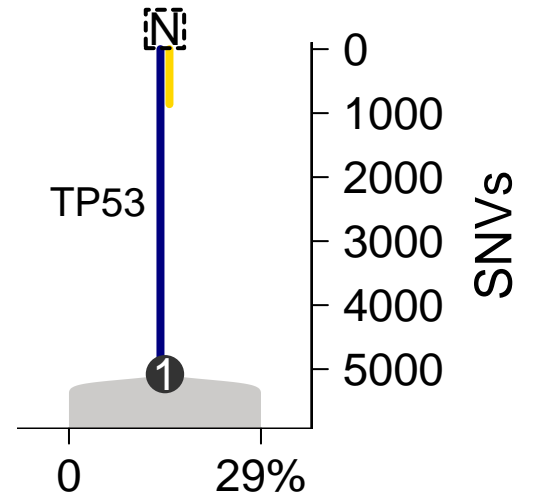
SomaticSniper-TITAN
