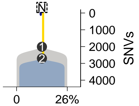
SomaticSniper-TITAN
