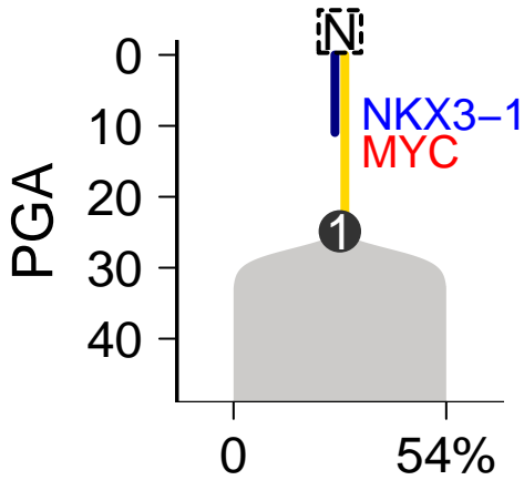
SomaticSniper-Battenberg
