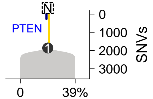
SomaticSniper-TITAN
