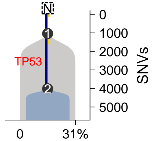
SomaticSniper-TITAN
