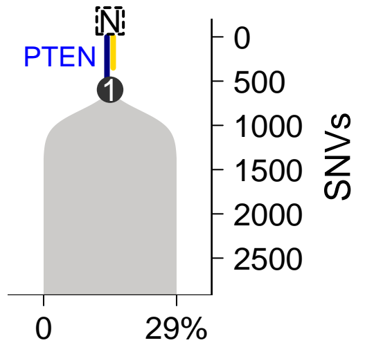
SomaticSniper–TITAN
