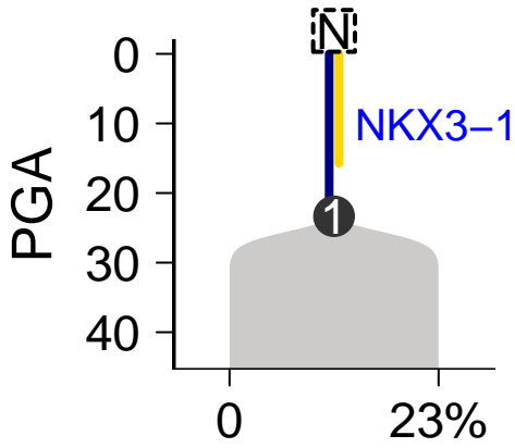
SomaticSniper-Battenberg
