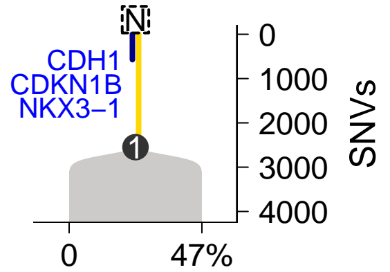
SomaticSniper-TITAN
