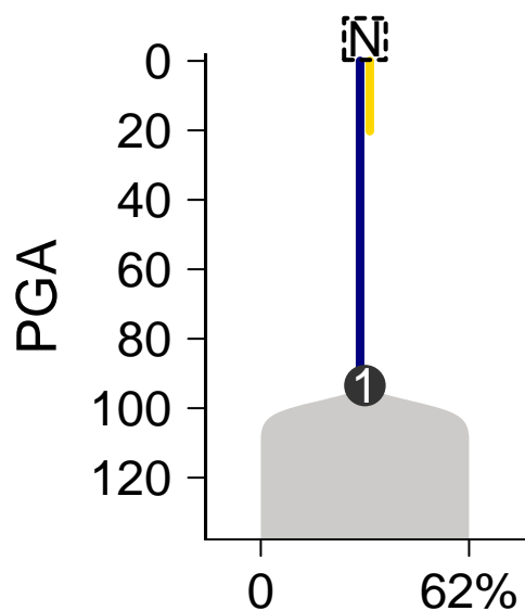
SomaticSniper-Battenberg
