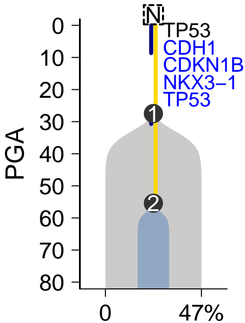
MuTect–Battenberg
