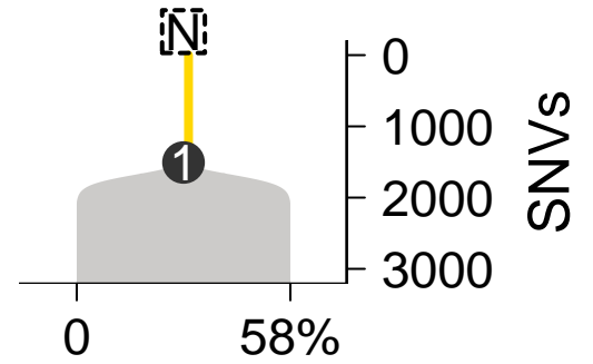
SomaticSniper-TITAN
