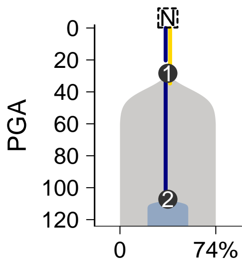
SomaticSniper-Battenberg
