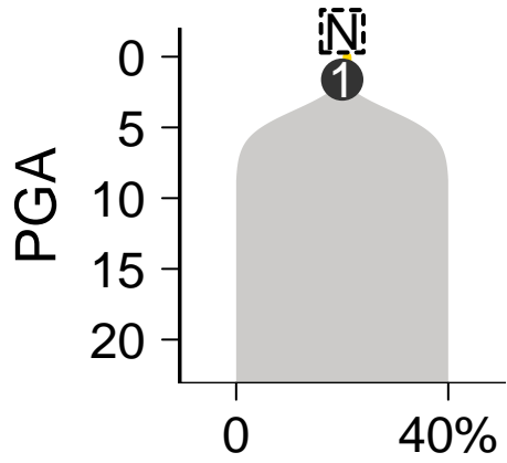
SomaticSniper-Battenberg
