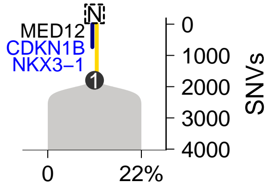
SomaticSniper-TITAN
