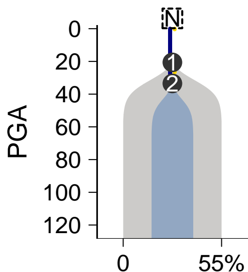
SomaticSniper-Battenberg
