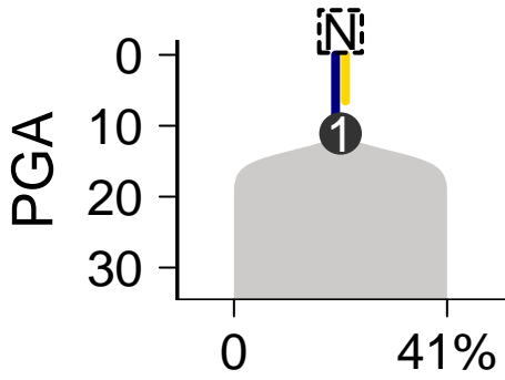
SomaticSniper-Battenberg
