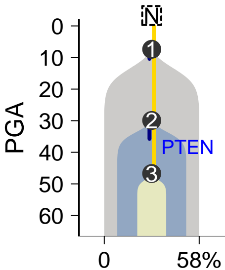
MuTect–Battenberg
