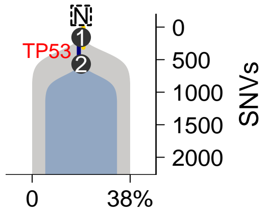
SomaticSniper–TITAN
