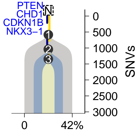
SomaticSniper-TITAN
