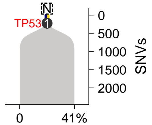
SomaticSniper-TITAN
