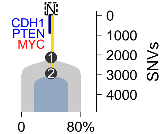
SomaticSniper-TITAN
