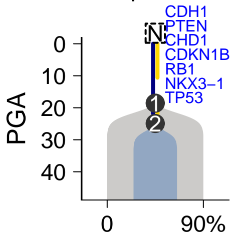
SomaticSniper-Battenberg
