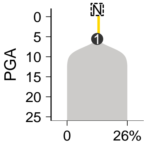
SomaticSniper-Battenberg
