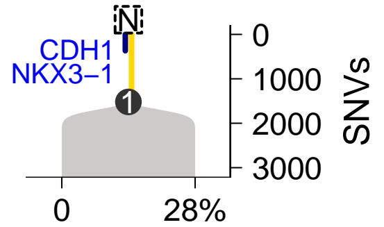
SomaticSniper-TITAN
