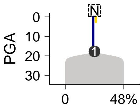
SomaticSniper-Battenberg
