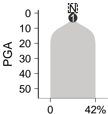
SomaticSniper-Battenberg
