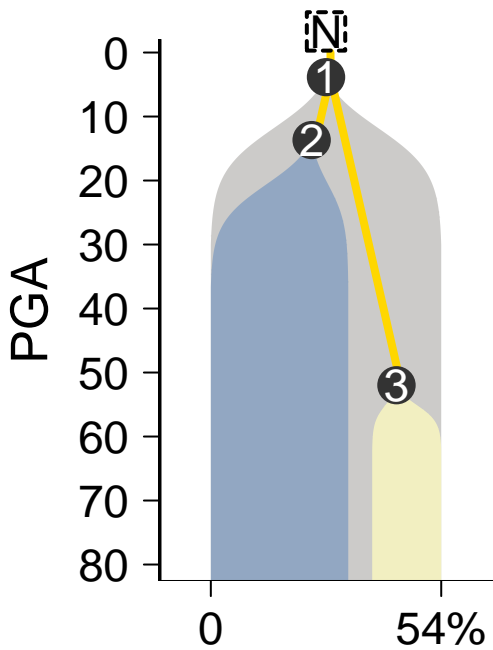
MuTect–Battenberg
