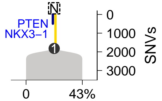
SomaticSniper–TITAN
