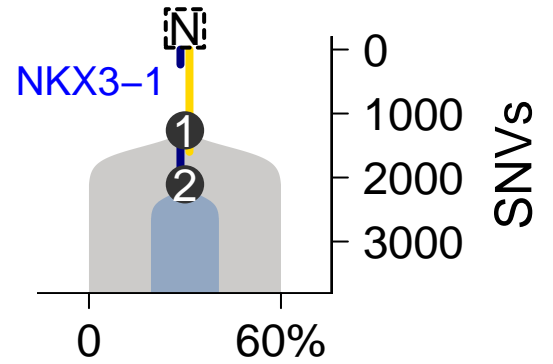
SomaticSniper-TITAN
