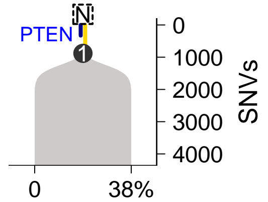
SomaticSniper-TITAN
