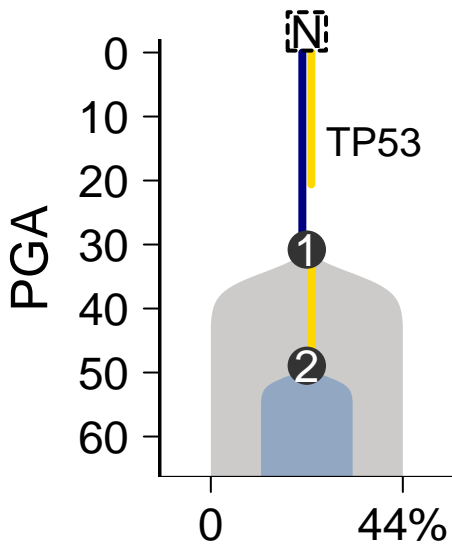
MuTect–Battenberg
