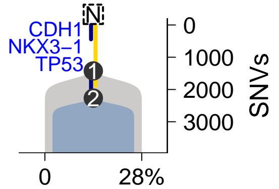
SomaticSniper–TITAN
