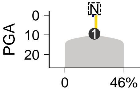
SomaticSniper-Battenberg
