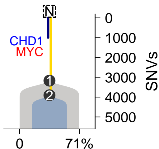
SomaticSniper-TITAN
