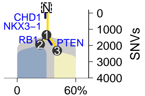
SomaticSniper-TITAN
