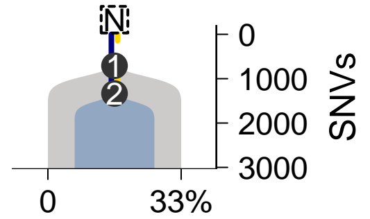
SomaticSniper-TITAN
