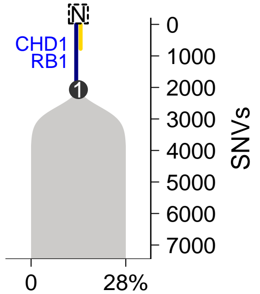
SomaticSniper-TITAN
