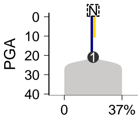
SomaticSniper-Battenberg
