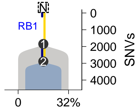
SomaticSniper-TITAN
