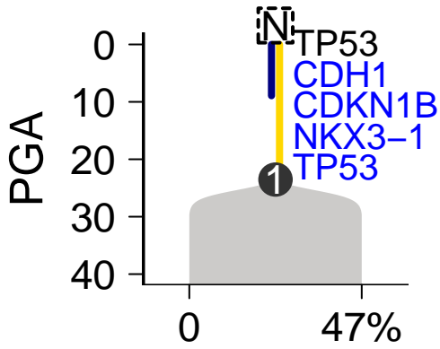
SomaticSniper–Battenberg
