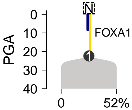
SomaticSniper-Battenberg
