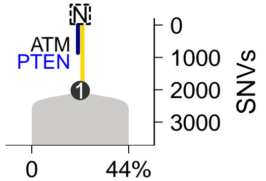
SomaticSniper-TITAN
