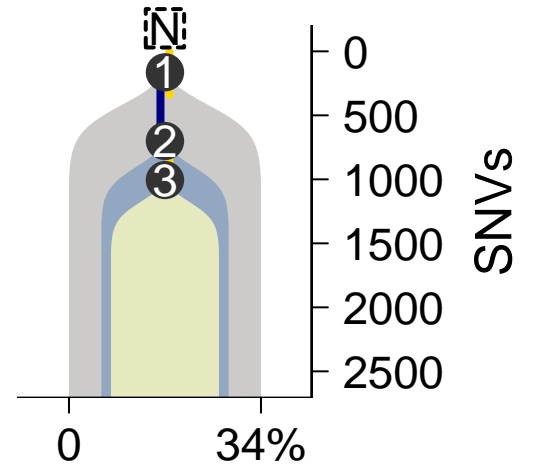
SomaticSniper-TITAN
