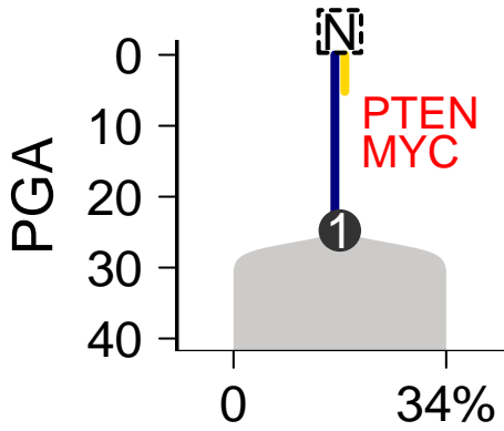
SomaticSniper-Battenberg
