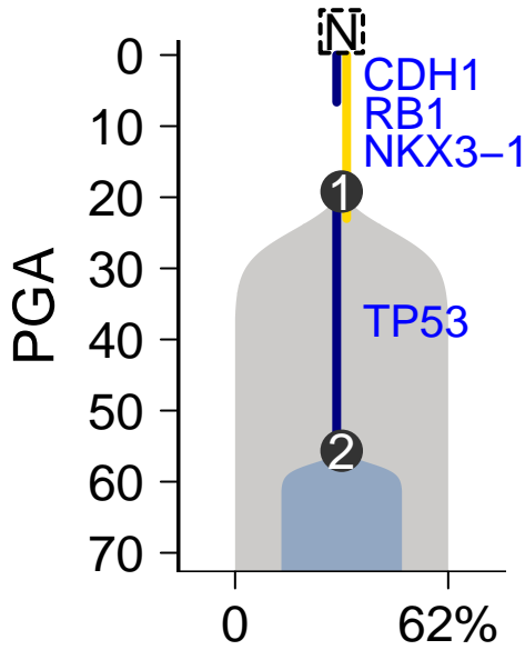
SomaticSniper-Battenberg
