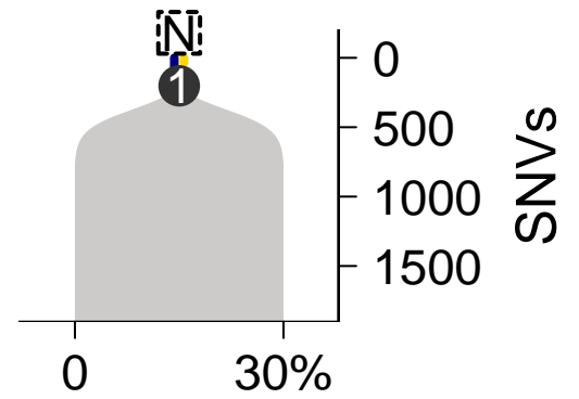
SomaticSniper-TITAN
