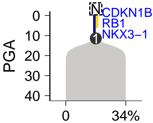
SomaticSniper-Battenberg
