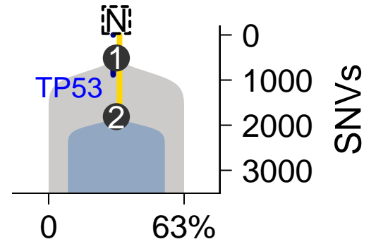
SomaticSniper-TITAN
