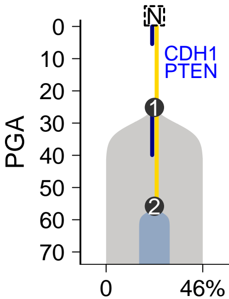
MuTect–Battenberg
