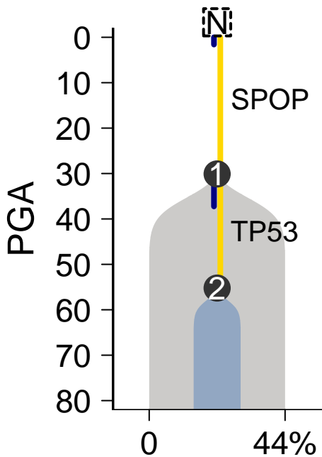
MuTect–Battenberg
