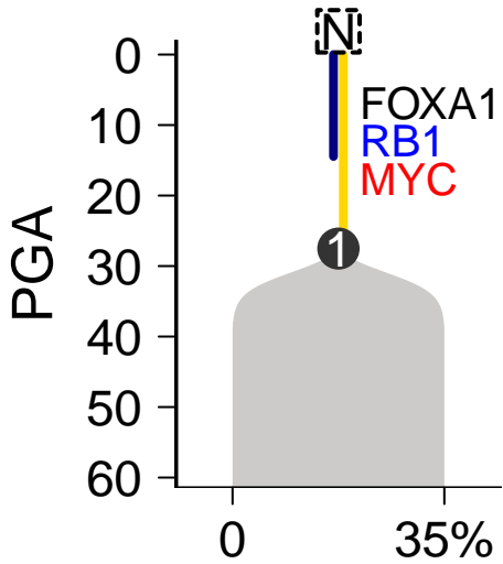
SomaticSniper-Battenberg
