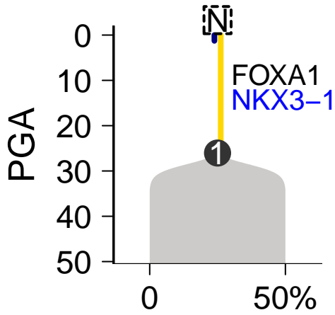
SomaticSniper-Battenberg
