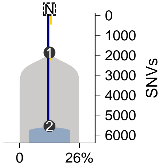
SomaticSniper-TITAN
