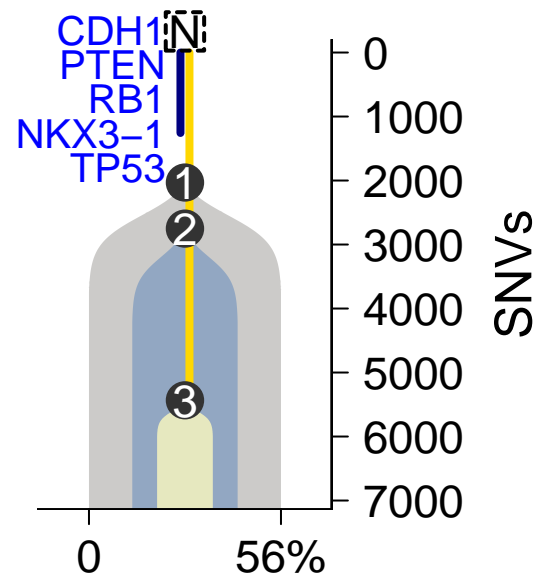
MuTect–TITAN
