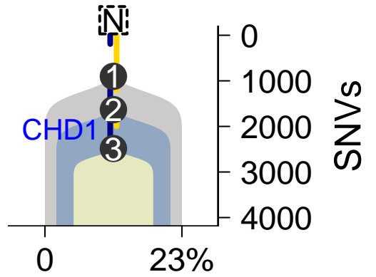
SomaticSniper–TITAN
