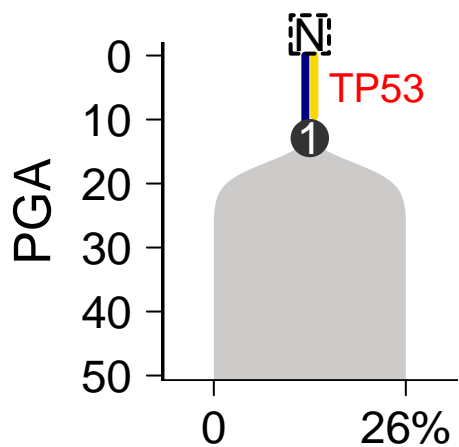
SomaticSniper-Battenberg
