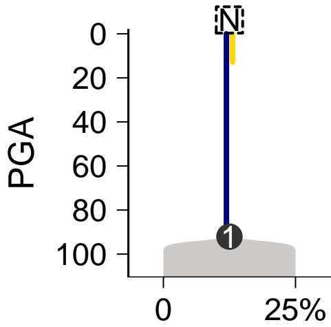
SomaticSniper-Battenberg
