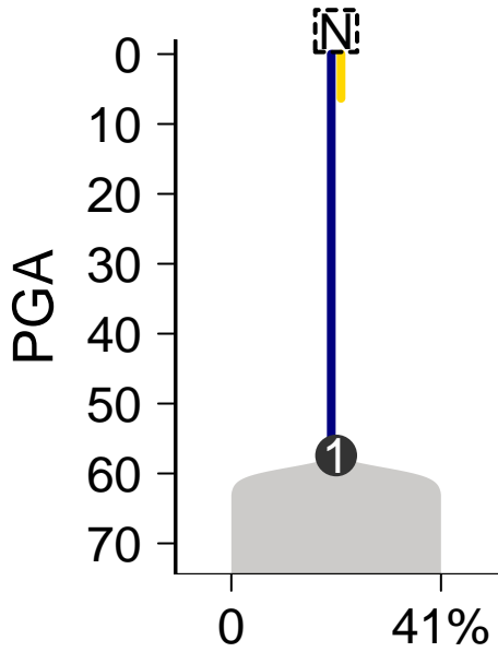
SomaticSniper-Battenberg
