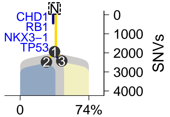
SomaticSniper-TITAN
