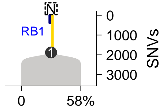
SomaticSniper-TITAN
