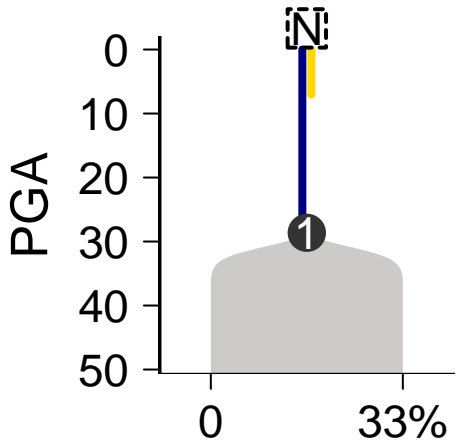
SomaticSniper-Battenberg
