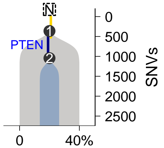
SomaticSniper–TITAN
