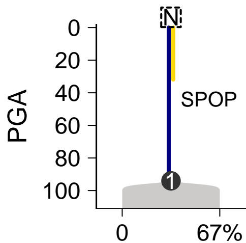
SomaticSniper-Battenberg
