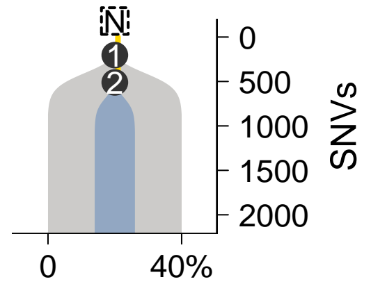
SomaticSniper-TITAN
