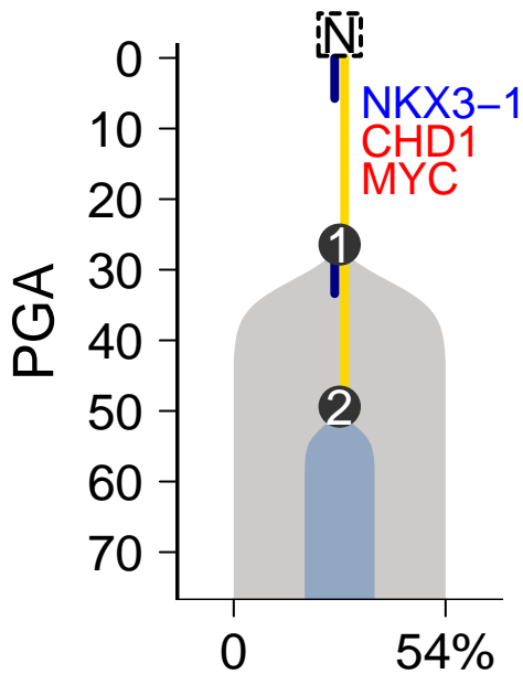
MuTect–Battenberg
