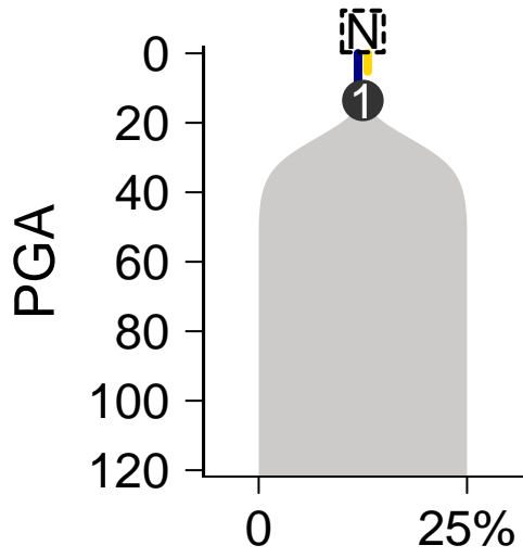
SomaticSniper-Battenberg
