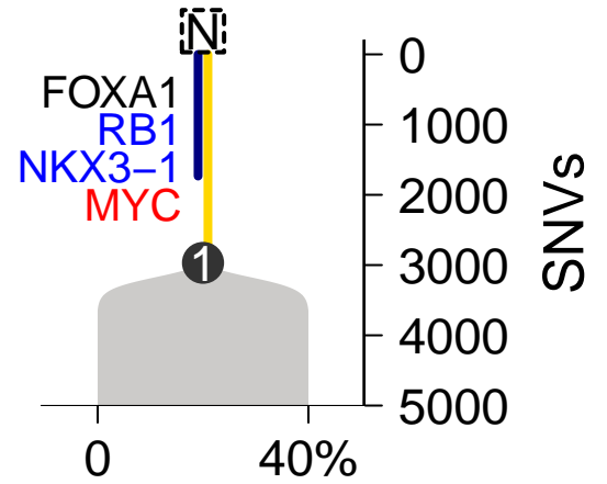
SomaticSniper-TITAN
