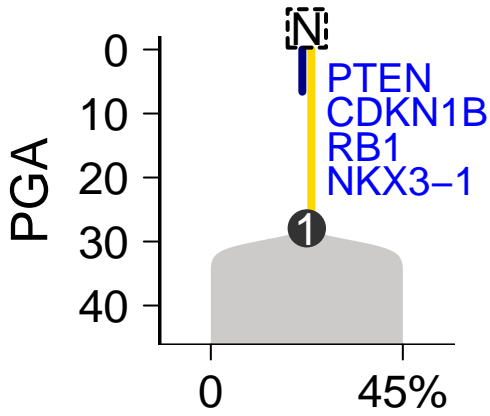
SomaticSniper-Battenberg
