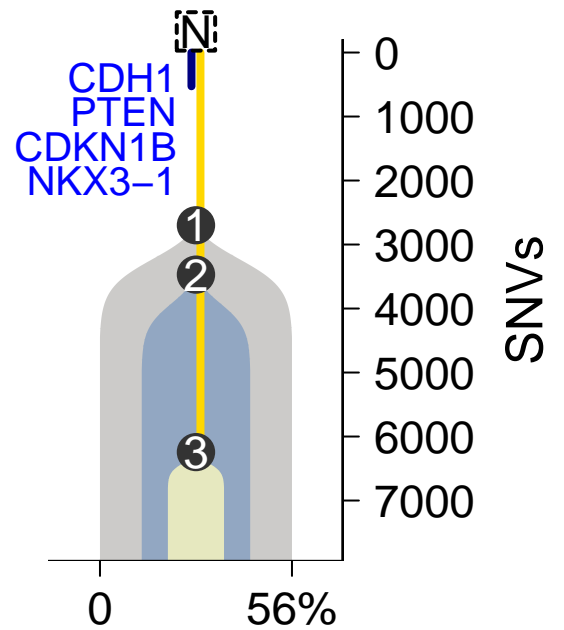
MuTect–TITAN
