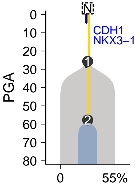
MuTect–Battenberg
