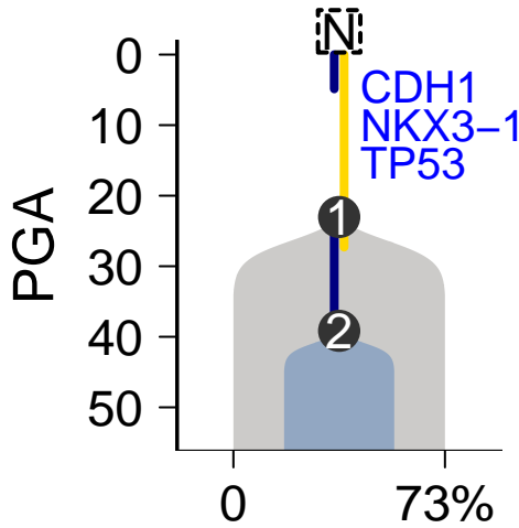
SomaticSniper-Battenberg
