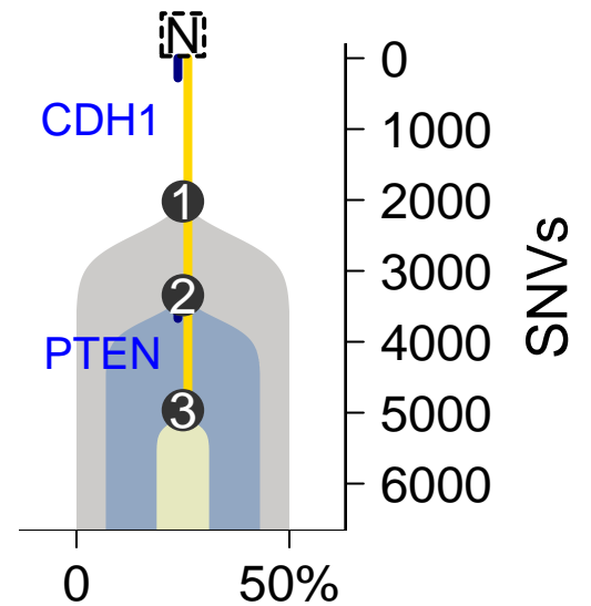
MuTect–TITAN
