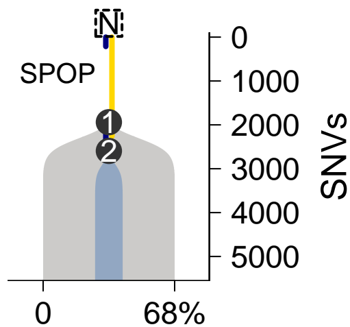
SomaticSniper-TITAN
