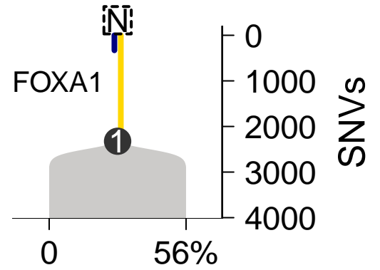
SomaticSniper-TITAN
