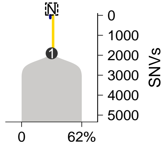
SomaticSniper-TITAN
