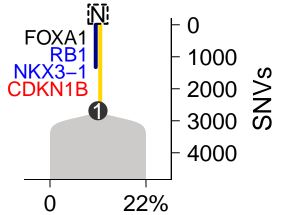
SomaticSniper-TITAN
