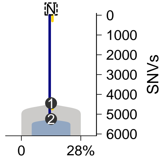
SomaticSniper-TITAN
