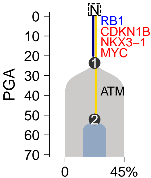
MuTect–Battenberg
