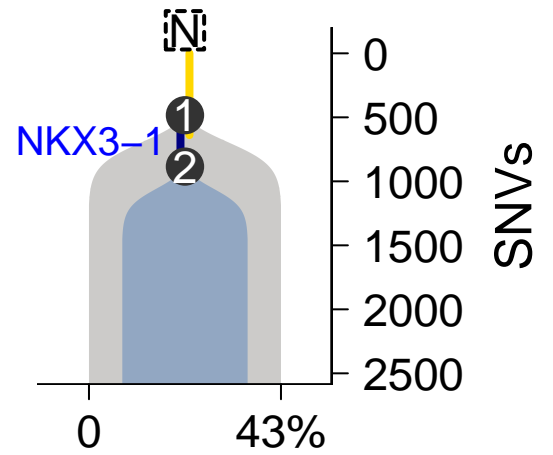
SomaticSniper–TITAN
