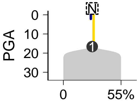
SomaticSniper-Battenberg
