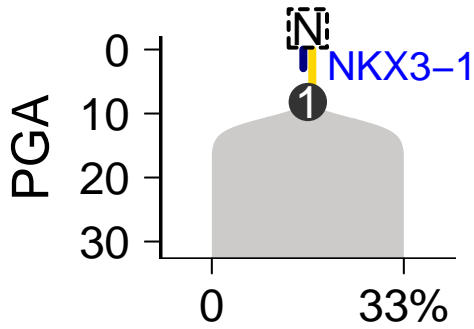
SomaticSniper-Battenberg
