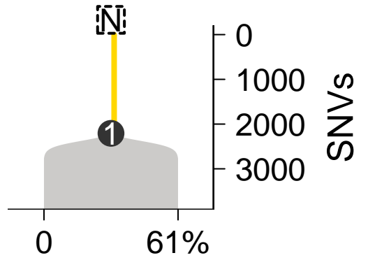
SomaticSniper-TITAN
