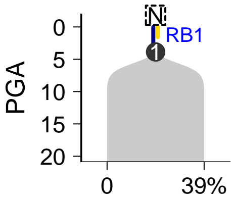
SomaticSniper-Battenberg
