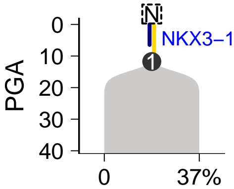
SomaticSniper-Battenberg
