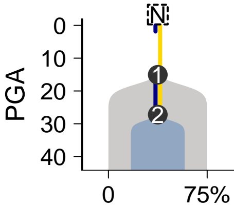
SomaticSniper-Battenberg
