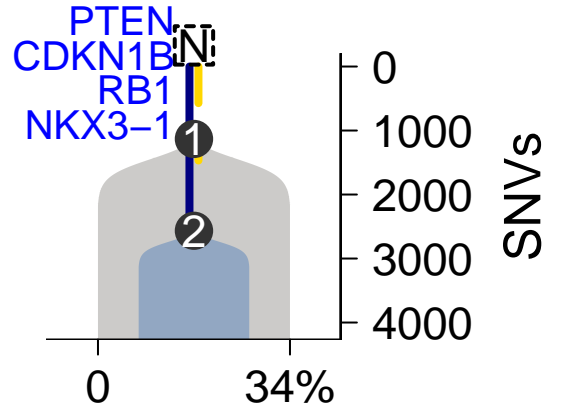
SomaticSniper-TITAN
