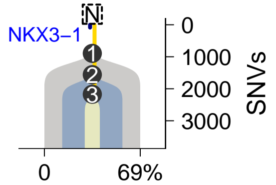
SomaticSniper-TITAN
