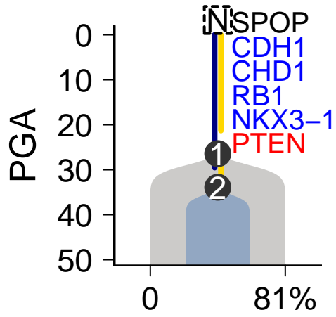
SomaticSniper-Battenberg
