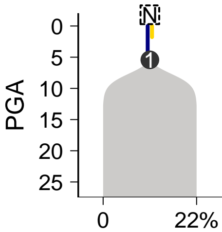
SomaticSniper–Battenberg
