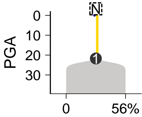
SomaticSniper-Battenberg
