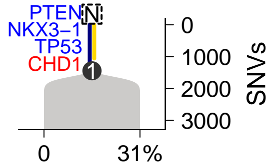
SomaticSniper-TITAN
