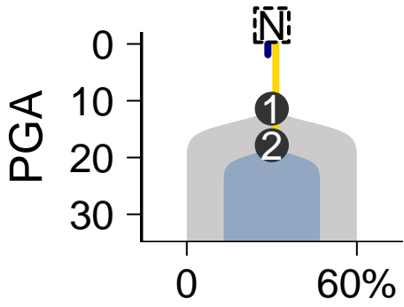
SomaticSniper-Battenberg
