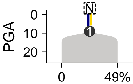
SomaticSniper-Battenberg
