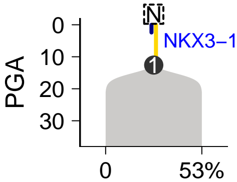
SomaticSniper-Battenberg
