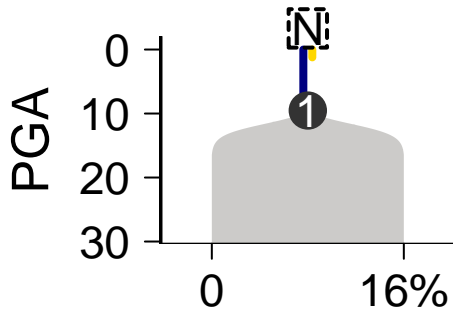
SomaticSniper-Battenberg
