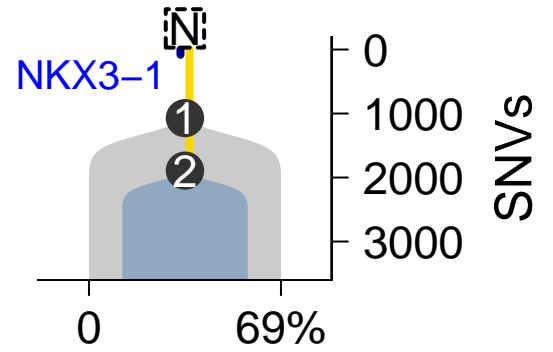
SomaticSniper-TITAN
