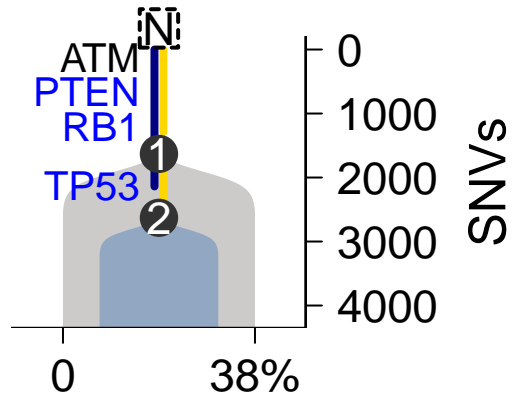
SomaticSniper-TITAN
