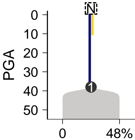
SomaticSniper-Battenberg
