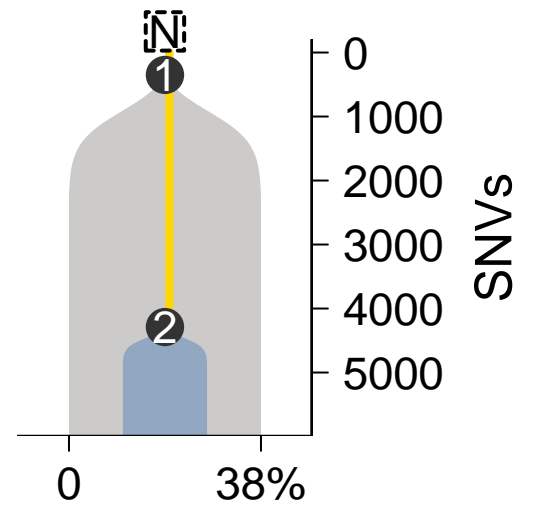
MuTect–TITAN
