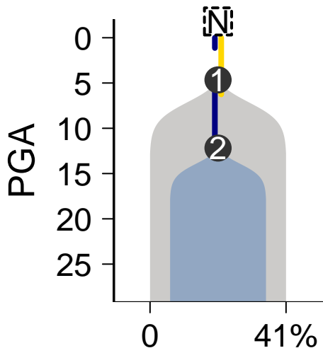
SomaticSniper–Battenberg
