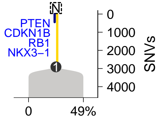
SomaticSniper-TITAN
