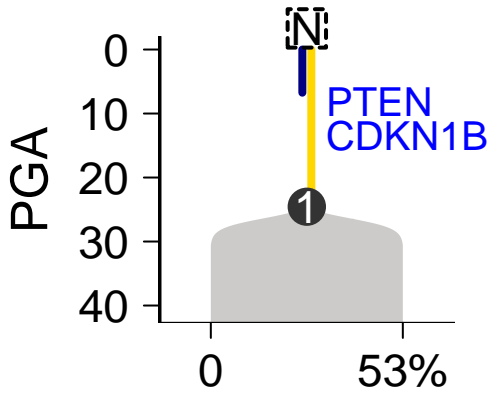
SomaticSniper–Battenberg
