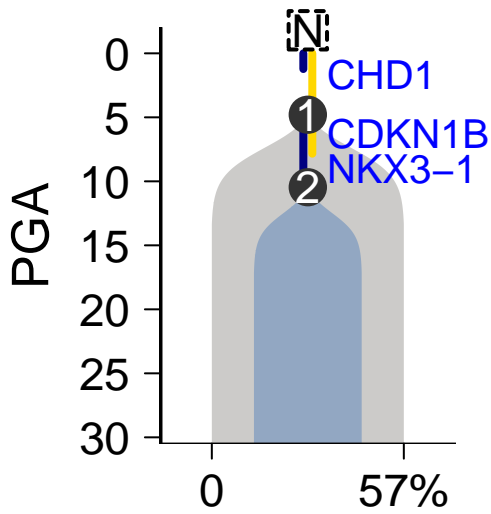
SomaticSniper-Battenberg
