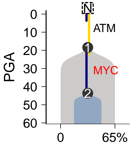
SomaticSniper-Battenberg
