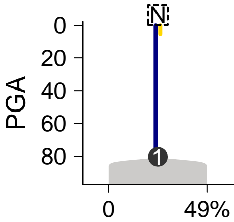
SomaticSniper-Battenberg
