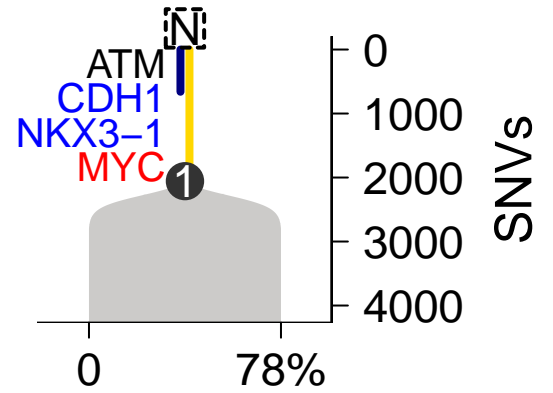
SomaticSniper-TITAN
