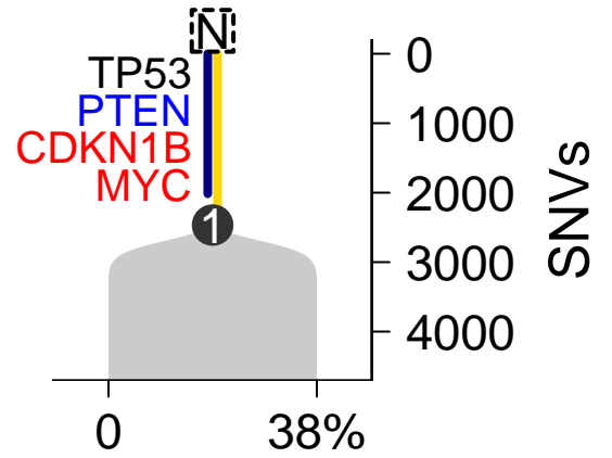
SomaticSniper-TITAN
