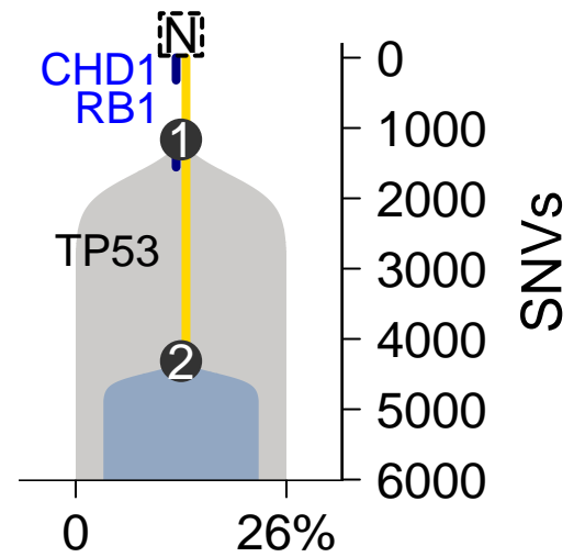
MuTect–TITAN
