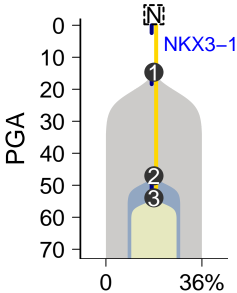
MuTect–Battenberg
