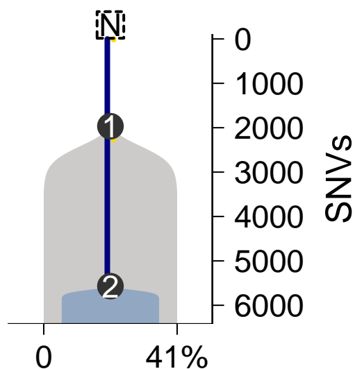
SomaticSniper-TITAN
