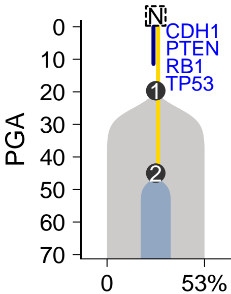
MuTect–Battenberg
