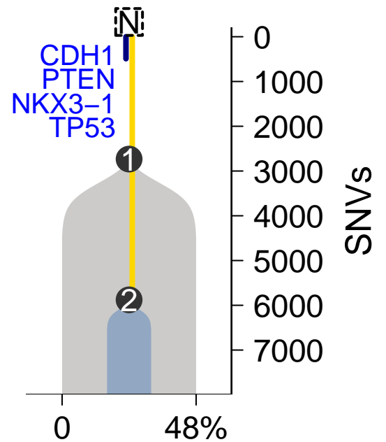
MuTect–TITAN
