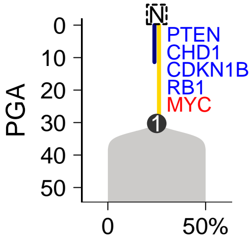
SomaticSniper–Battenberg
