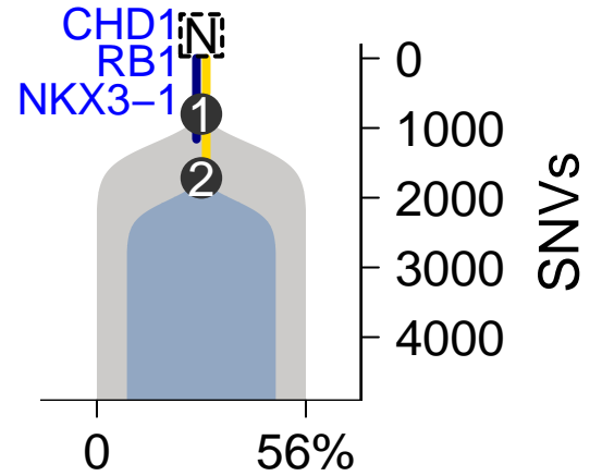
SomaticSniper-TITAN
