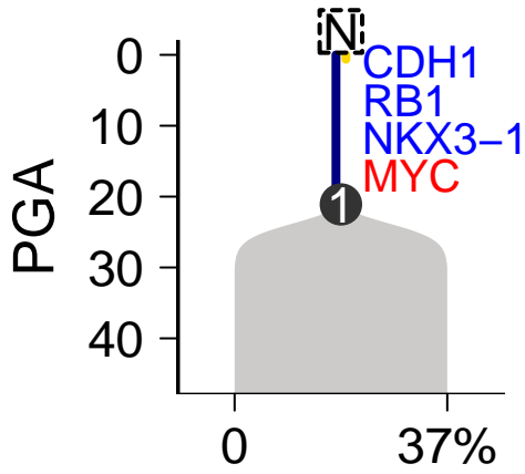
SomaticSniper–Battenberg
