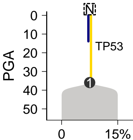
MuTect–Battenberg
