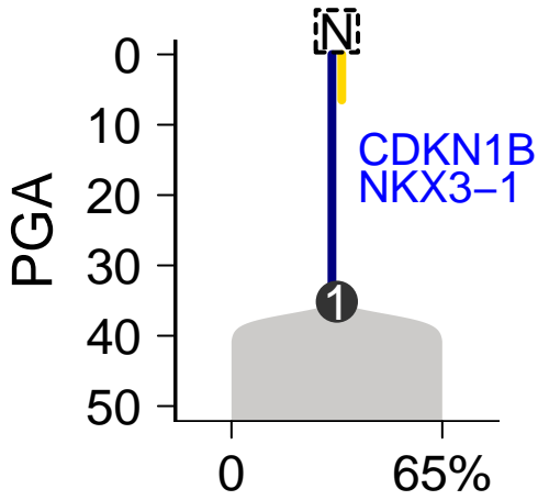
SomaticSniper-Battenberg
