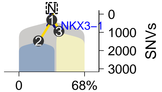
SomaticSniper-TITAN
