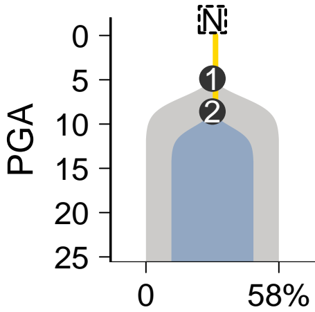
SomaticSniper-Battenberg
