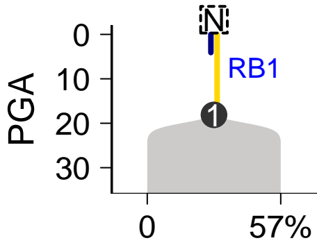
SomaticSniper-Battenberg
