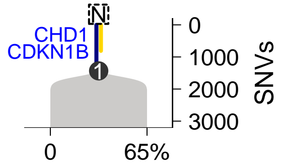
SomaticSniper-TITAN
