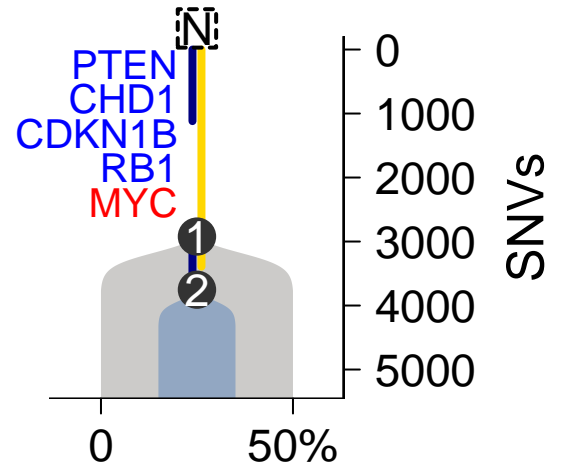
SomaticSniper–TITAN
