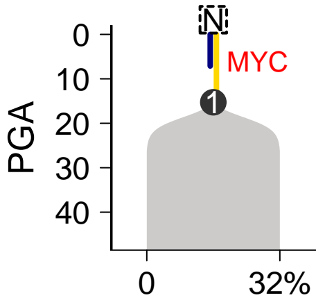
SomaticSniper-Battenberg
