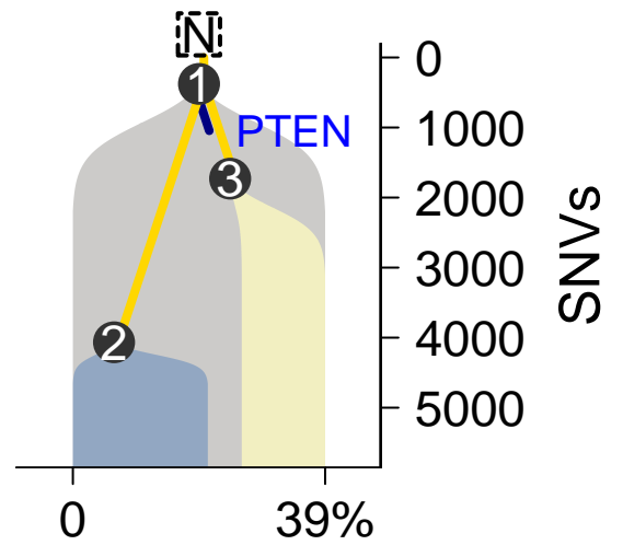
MuTect–TITAN
