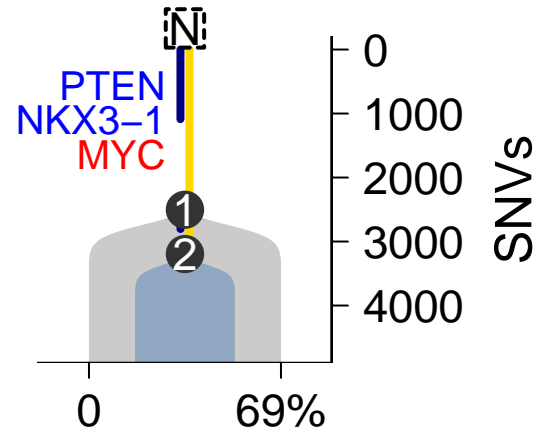
SomaticSniper-TITAN
