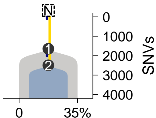
SomaticSniper-TITAN
