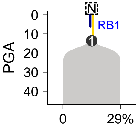
SomaticSniper-Battenberg
