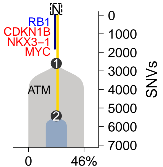
MuTect–TITAN
