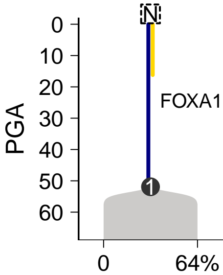
SomaticSniper-Battenberg
