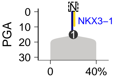
SomaticSniper-Battenberg
