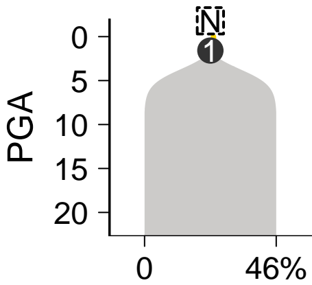
SomaticSniper–Battenberg
