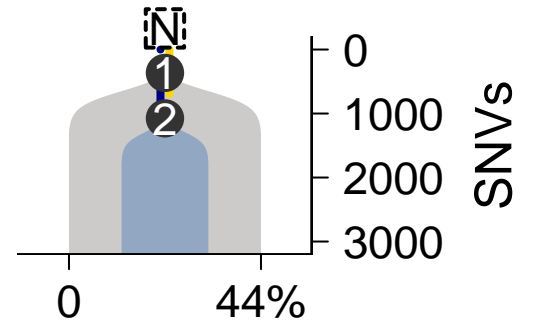
SomaticSniper-TITAN
