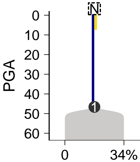
SomaticSniper-Battenberg
