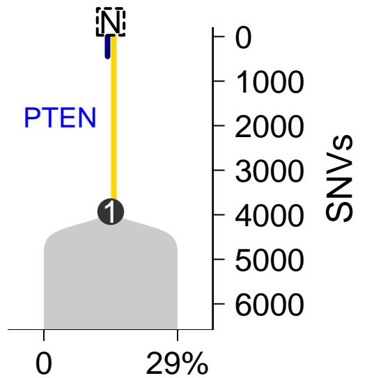
MuTect–TITAN
