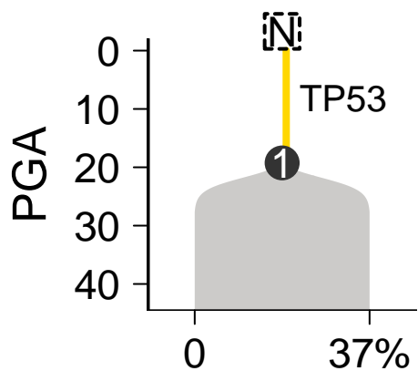
SomaticSniper-Battenberg
