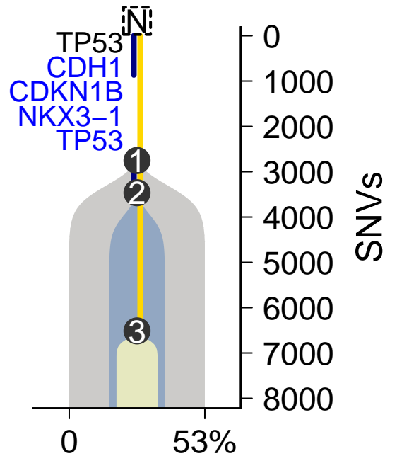
MuTect–TITAN
