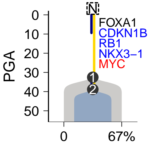
SomaticSniper–Battenberg
