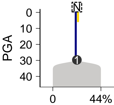
SomaticSniper-Battenberg
