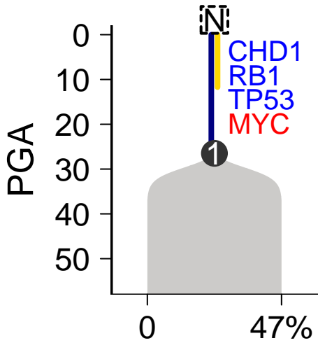
SomaticSniper-Battenberg
