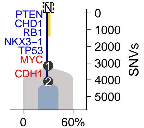
SomaticSniper-TITAN
