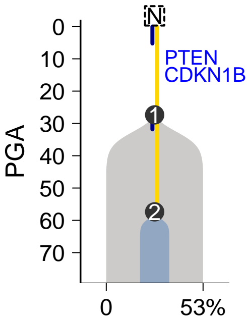
MuTect–Battenberg
