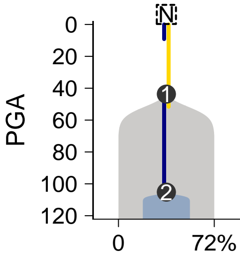
SomaticSniper-Battenberg
