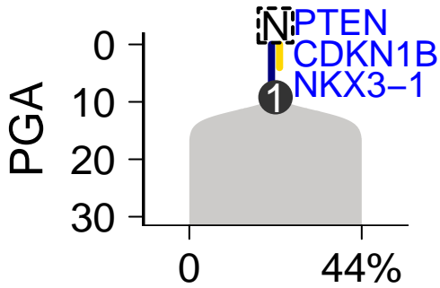
SomaticSniper–Battenberg
