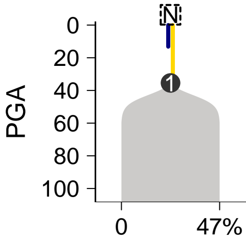
SomaticSniper-Battenberg
