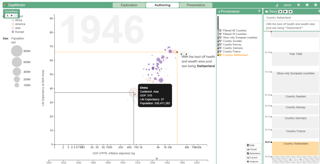
Figure 3: Screenshot of the GapMinder-inspired application in authoring mode showing the combination of selection with annotation and custom mouse interaction.
