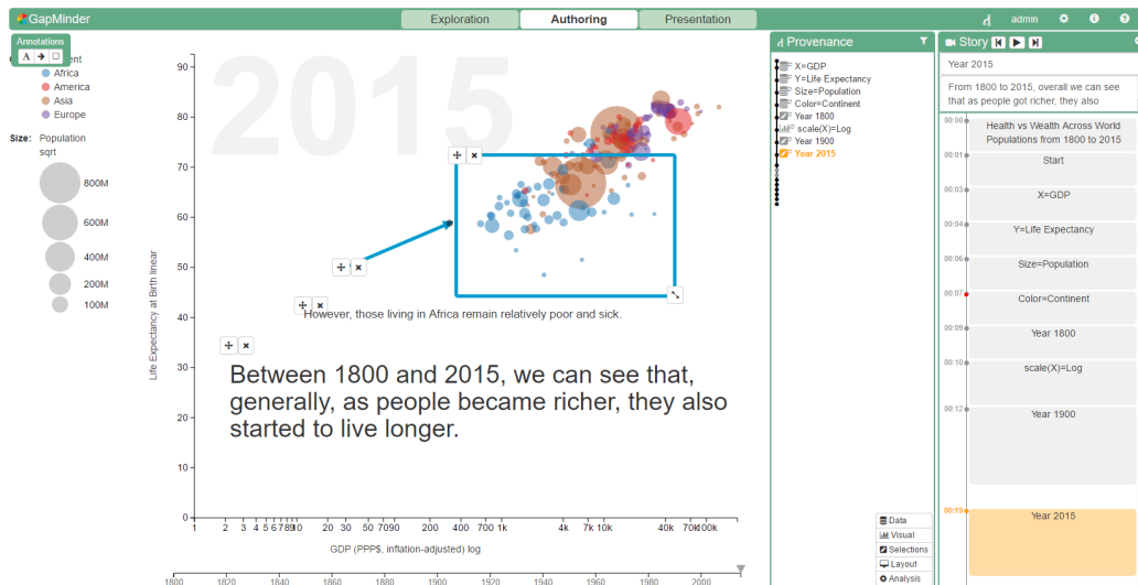
Figure 1: Screenshot of the Gapminder-inspired application showing the same state as the usage scenario in authoring mode.
