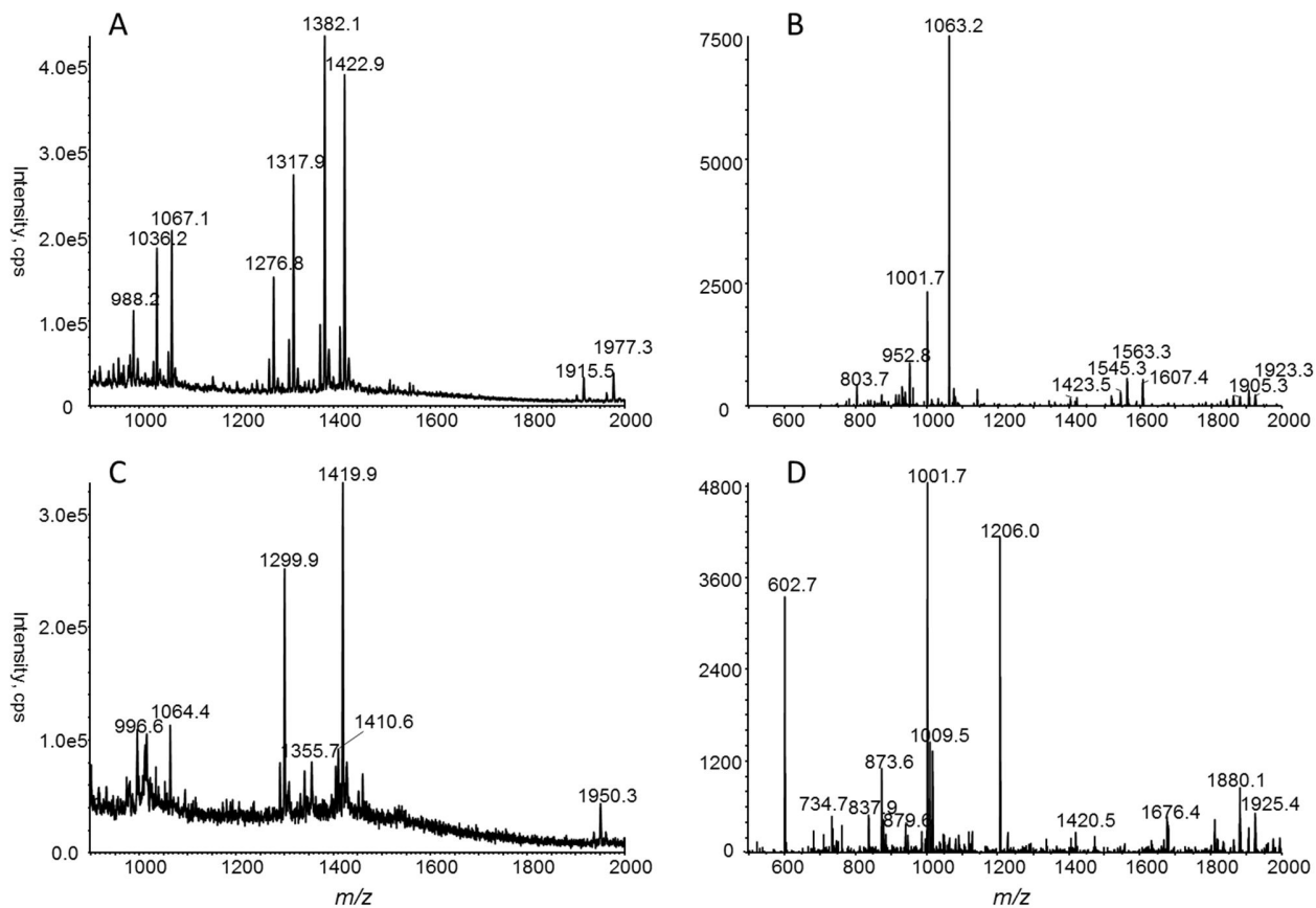
Supplemental Figure 1. Example of the electrophoresis-assisted open-tubular liquid chromatography electrospray mass spectrometry (EA-OTLC-MS) analysis of intact LOS from C. coli . (A) extracted mass spectrum for strain #137; (B) extracted MS/MS spectrum for precursor ion at m/z 1422.9; (C) extracted mass spectrum for strain #65; (D) extracted MS/MS spectrum for precursor ion at m/z 1299.9.
