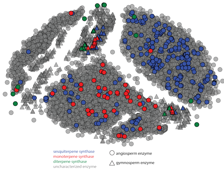
Figure S2: MDS plot of terpene synthase C-terminal domain sub-sequences with coloring based on substrate. Unknown proteins which are likely to be terpene synthases are shown in gray. Sequences which are similar to each other are closer together in the plot.
