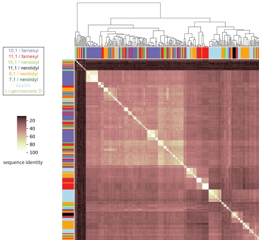
Figure S1: Visualization of C-terminal domain sequence identities between pairs of enzymes in the database. Colours on axes represent the major product precursor cations of the respective enzymes.
