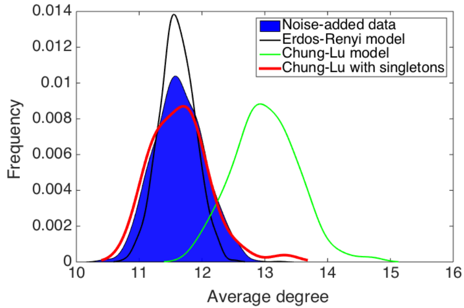
Supplemental Figure 2: Average degree in null models vs. noise-added data. This figure shows the Chung-Lu random graph has an artificially inflated average degree. This is due to the removal of singletons from the graph (red line includes singletons in the degree calculation; green line excludes them).
