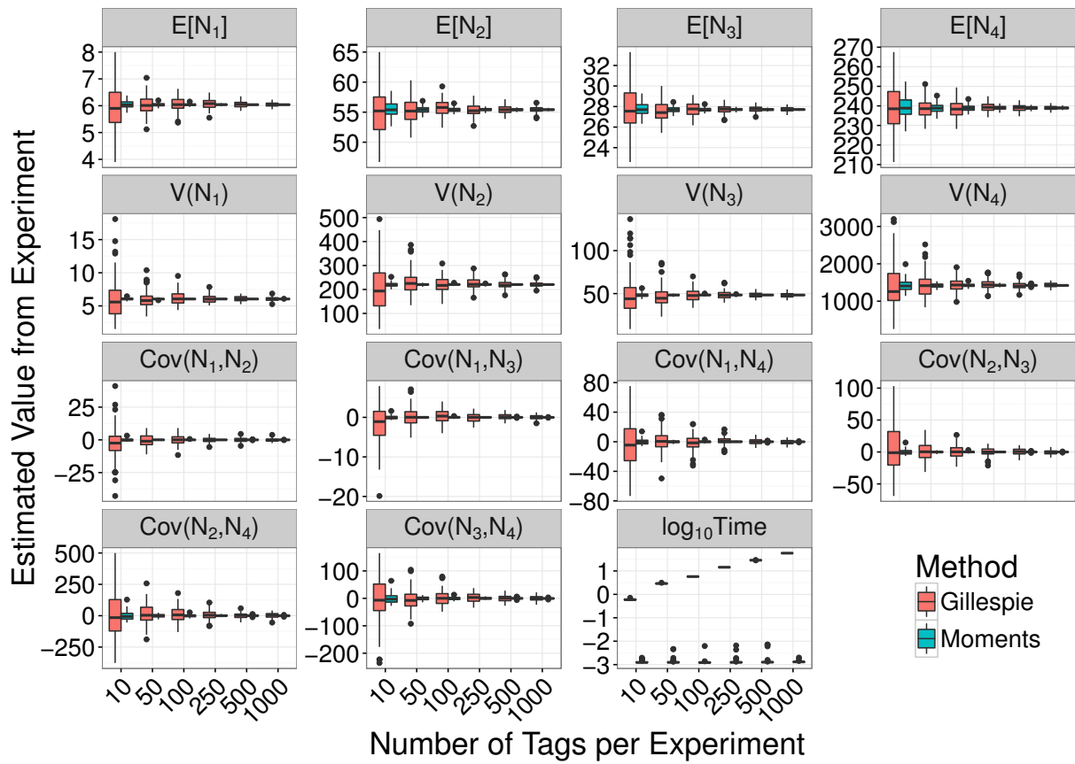
Figure S1: Box plots of estimated moments and log computation time from 100 simulated experiments of the radial network with four compartments, each of size 10, 50, 100, 250, 500 or 1000, calculated from the simulations and from the moments equations using the initial conditions.
