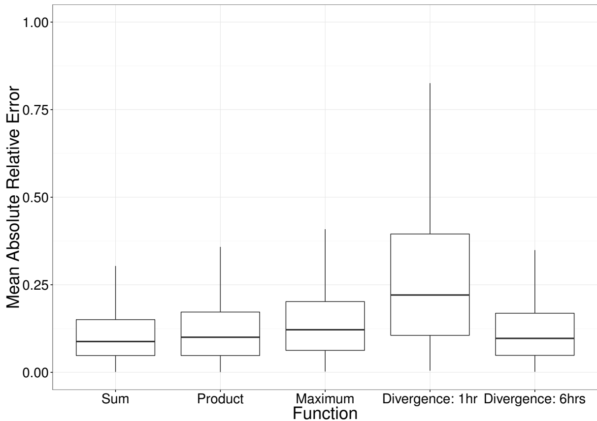
Figure S7: Box plots of the Mean Absolute Relative Error of parameter estimates for each divergence summary.
