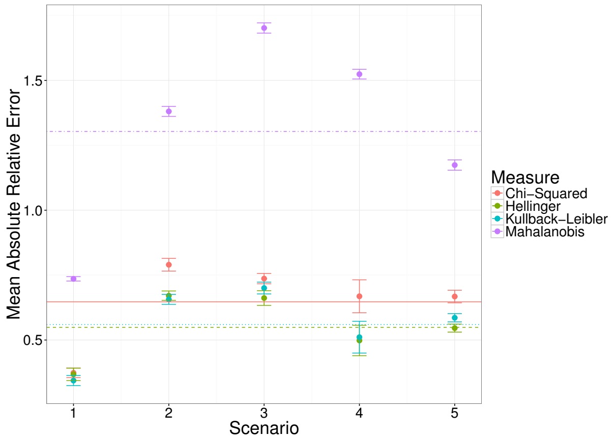
Figure S5: Mean Absolute Relative Error of parameter estimates of the radial model, for each divergence measure across each scenario, averaged across each of the 100 simulations at each observation time. The horizontal lines correspond to the average mean absolute relative error for each method.
