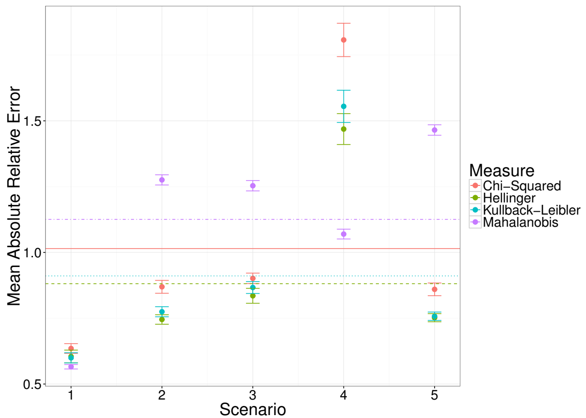
Figure S4: Mean Absolute Relative Error of parameter estimates of the linear model, for each divergence measure across each scenario, averaged across each of the 100 simulations at each observation time. The horizontal lines correspond to the average mean absolute relative error for each method.
