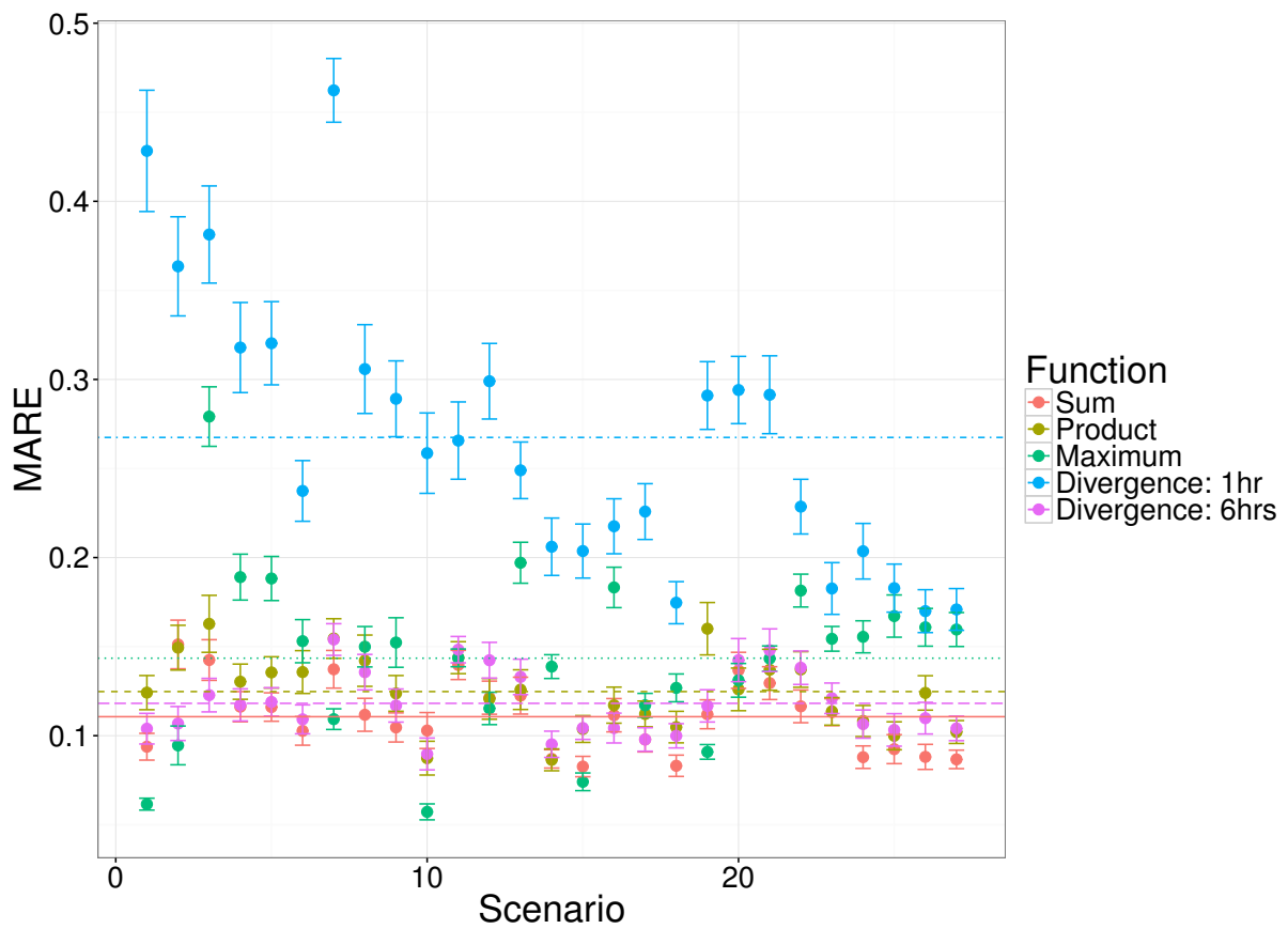
Figure S6: Mean Absolute Relative Error of parameter estimates for each divergence composition function across each scenario. The error bars represent \pm one standard error across the 100 simulations under each scenario. The horizontal lines correspond to the overall mean for each composition function.
