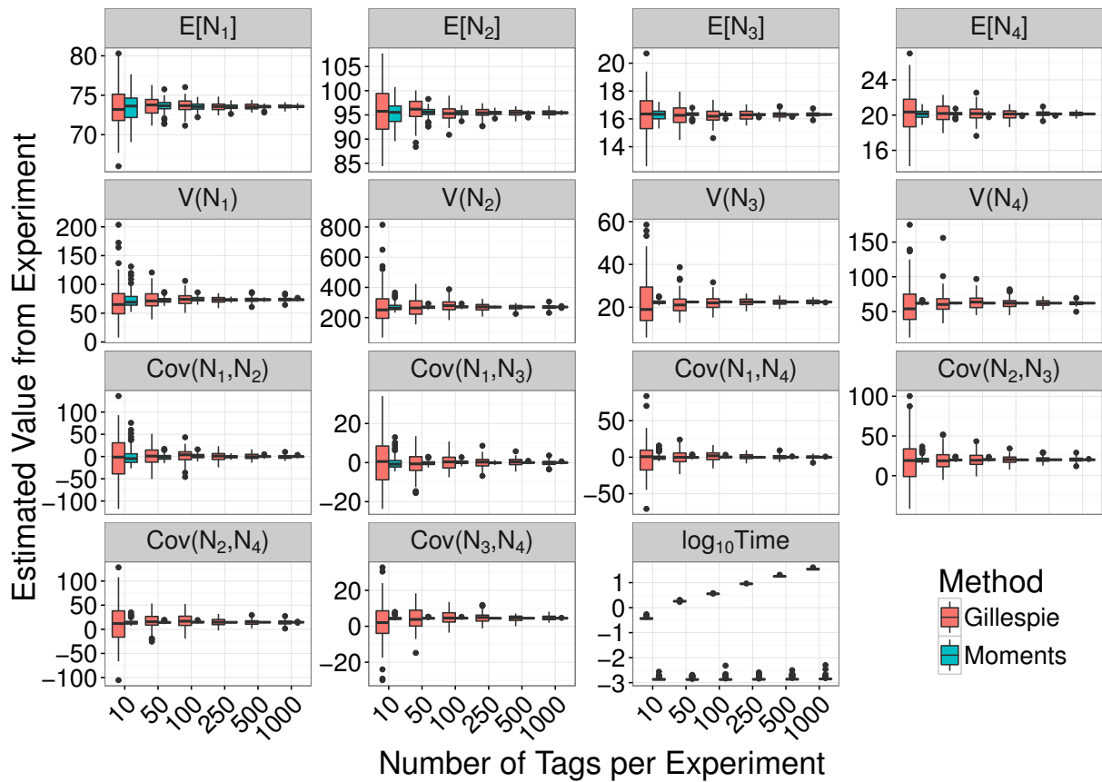
Figure S2: Box plots of estimated moments from 100 simulated experiments of the linear network with four compartments, each of size 10, 50, 100, 250, 500 or 1000, calculated from the simulations and from the moments equations using the initial conditions.
