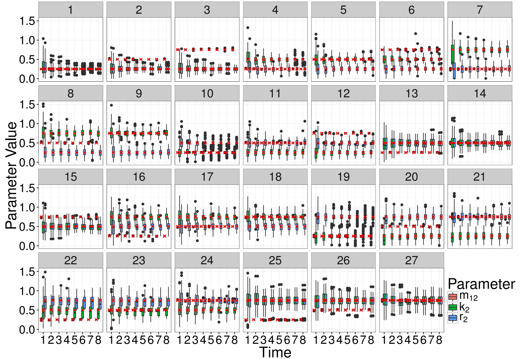
Figure S8: Box plots of MDE estimates corresponding to simulated data at \tau_1 = 2 , where the true parameter is denoted by the red cross.
