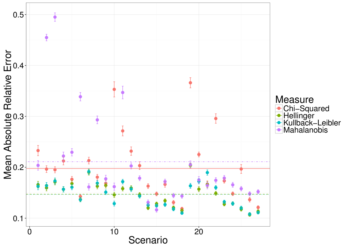
Figure S3: Mean Absolute Relative Error of parameter estimates of the simple model, for each divergence measure across each scenario, averaged across each of the 100 simulations at each observation time. The horizontal lines correspond to the average mean absolute relative error for each method.
