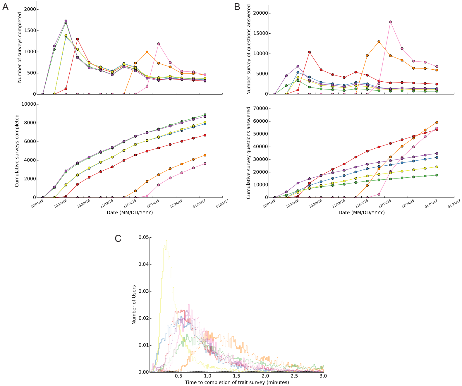
Supplementary Figure 3: Participation rates in DNA.Land’s trait prediction feature. Traits are predicted according to published GWAS summary statistics. (A) Per-week and cumulative numbers of total surveys completed by users. (B) Per-week and cumulative numbers of total questions answered by users. (C) The distribution of time required by users to complete each type of survey. The surveyed traits are as follows: (Orange) Chronotype, (Blue) Coffee Consumption, (Red) Myopia, (Green) Eye Color, (Pink) Neuroticism, (Purple) Educational Attainment, and (Yellow) Height.
