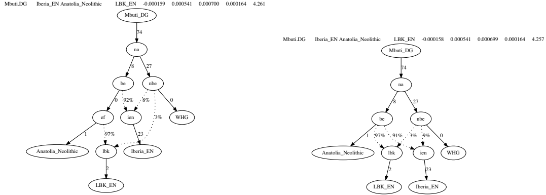
Figure S3.2: Systematic local searching to check alternative Admixture Graphs. Two modifications of the graph shown in Figure S3.1 that can be rejected. Left; the graph supported by naïve D statistics where Iberia_EN is an outgroup to Anatolia_Neolithic and LBK_EN. Right; a graph where the Early Farmer ancestry in the three Neolithic populations trifurcates. These two topologies actually lead to the same models, since one of the drift edges in the left model is fitted as 0 and are both rejected with Z=4.3 . We have not modeled alternative sources of hunter-gatherer ancestry, which could affect these graphs, but we know from PCA and ADMIXTURE analysis that the majority of the hunter-gatherer ancestry in Iberia_EN and LBK_EN is consistent with a WHG source.
