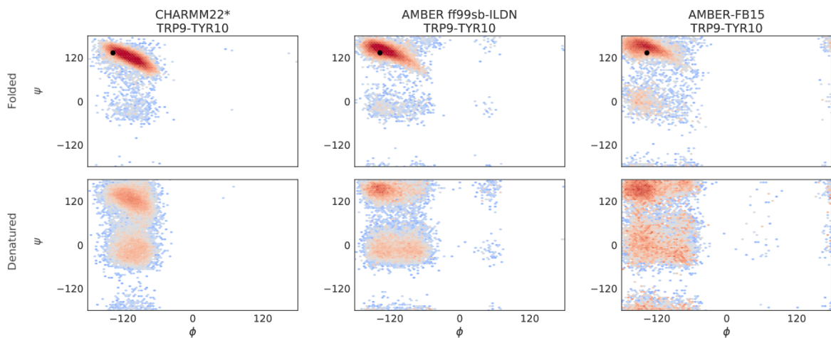
FIG. S7. Distribution of backbone dihedral angles as a function of force field, residue pair, and ensemble.
