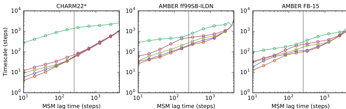
FIG. S13. Implied timescales for turn formation. The line at 50 ns indicates the lag time at which the model was optimized and used for analysis. Steps are 200 ps.
