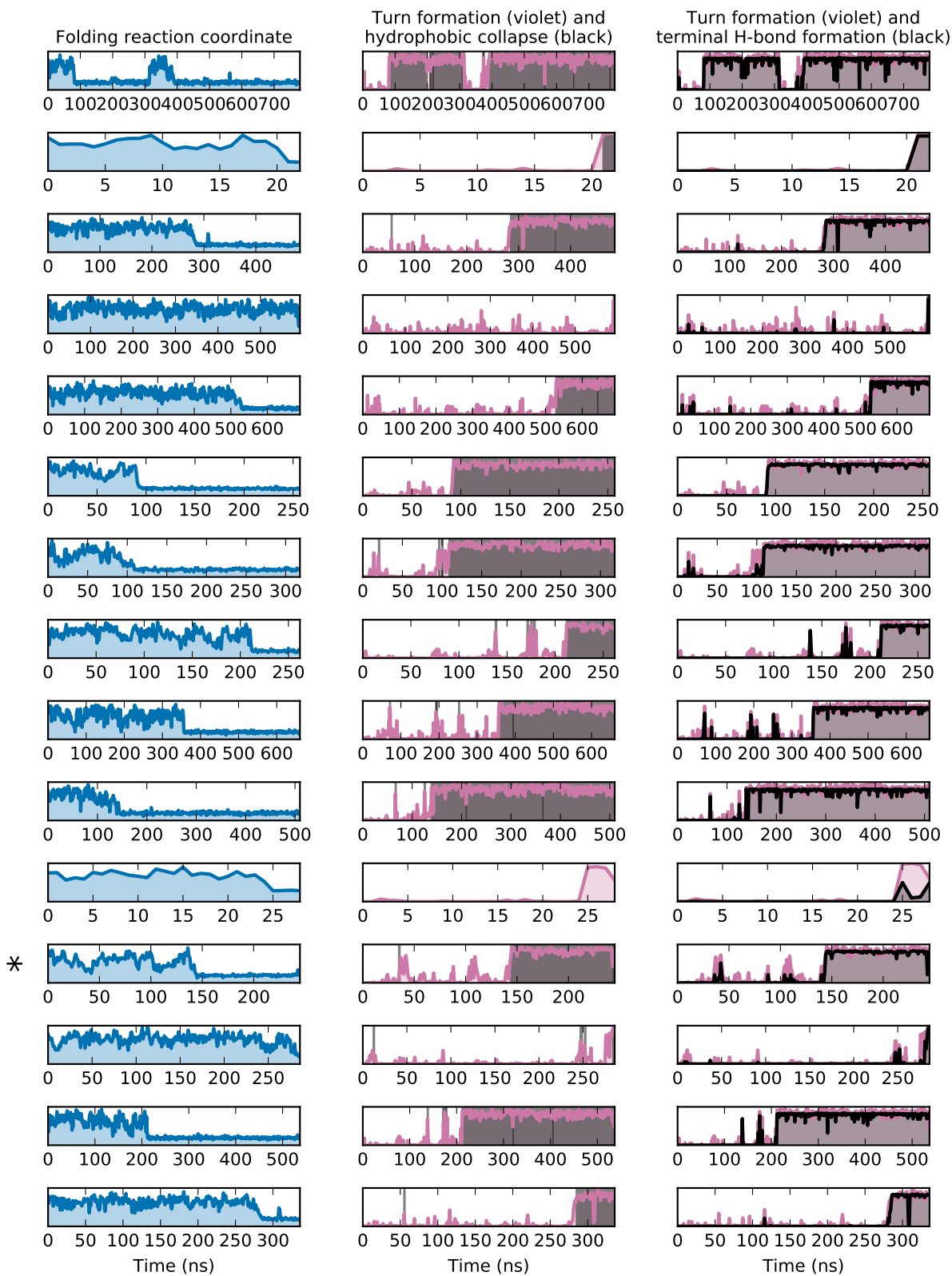
FIG. S8. 15 trajectories for CHARMM22* from the top 3 paths.
