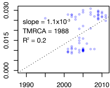
Mycobacterium tuberculosis Lineage 2
