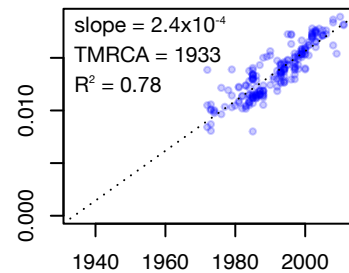
Shigella dysenteriae type 1 lineage IV
