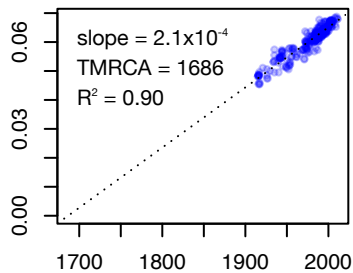
Shigella dysenteriae type 1 (global data set)
