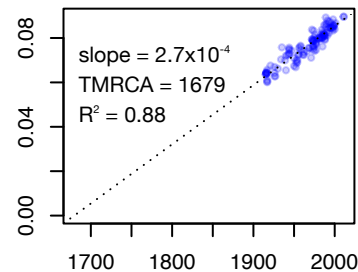
Shigella dysenteriae type 1
