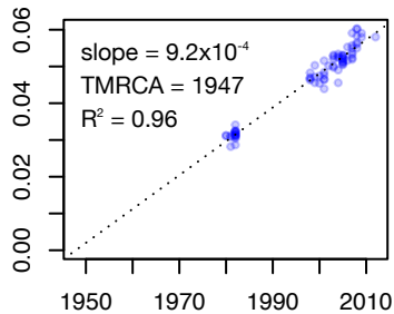
Staphylococcus aureus ST239
