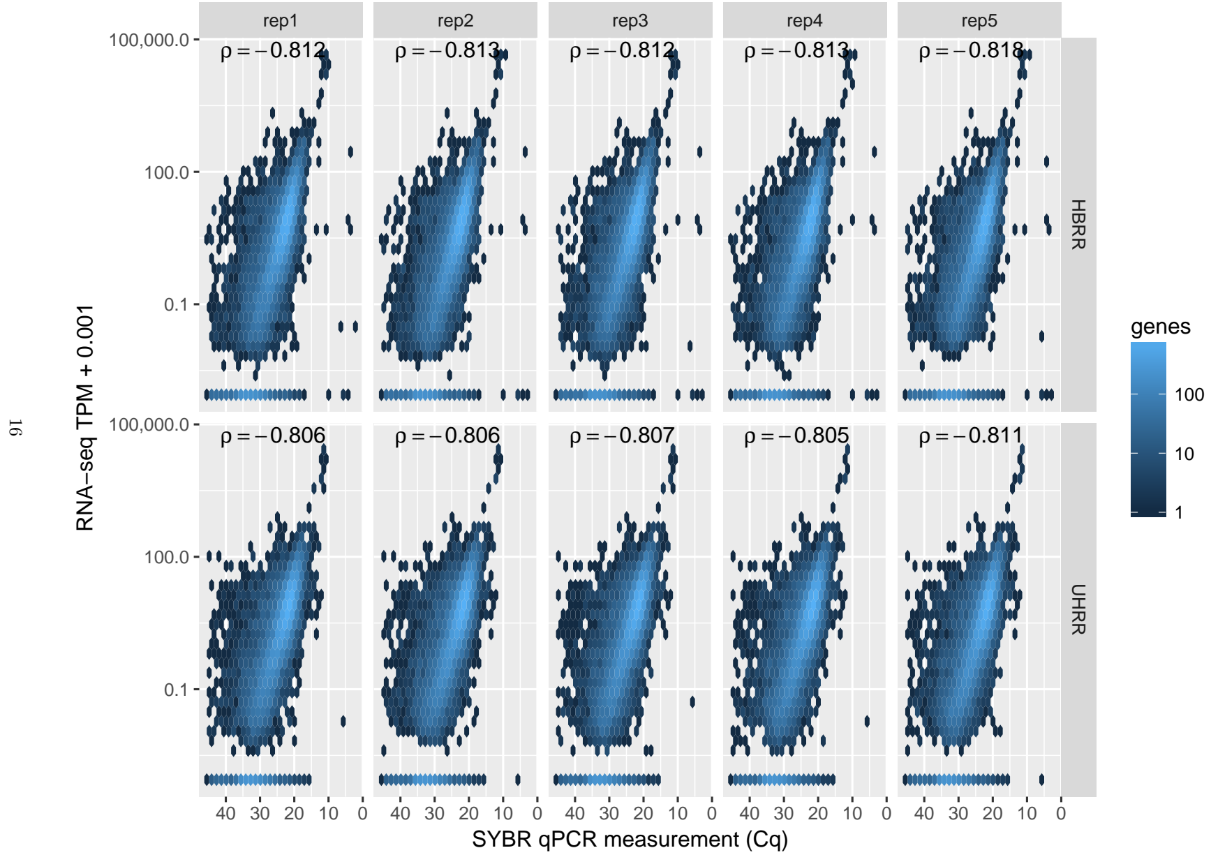
Figure S15: Correspondence of RNA-seq results with SYBR qPCR measurements.
