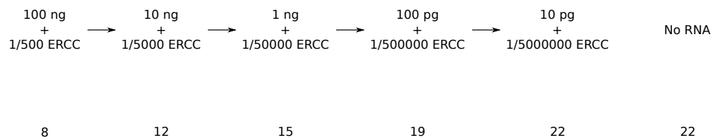
Figure S9: Experimental design of validation with human reference RNAs.
