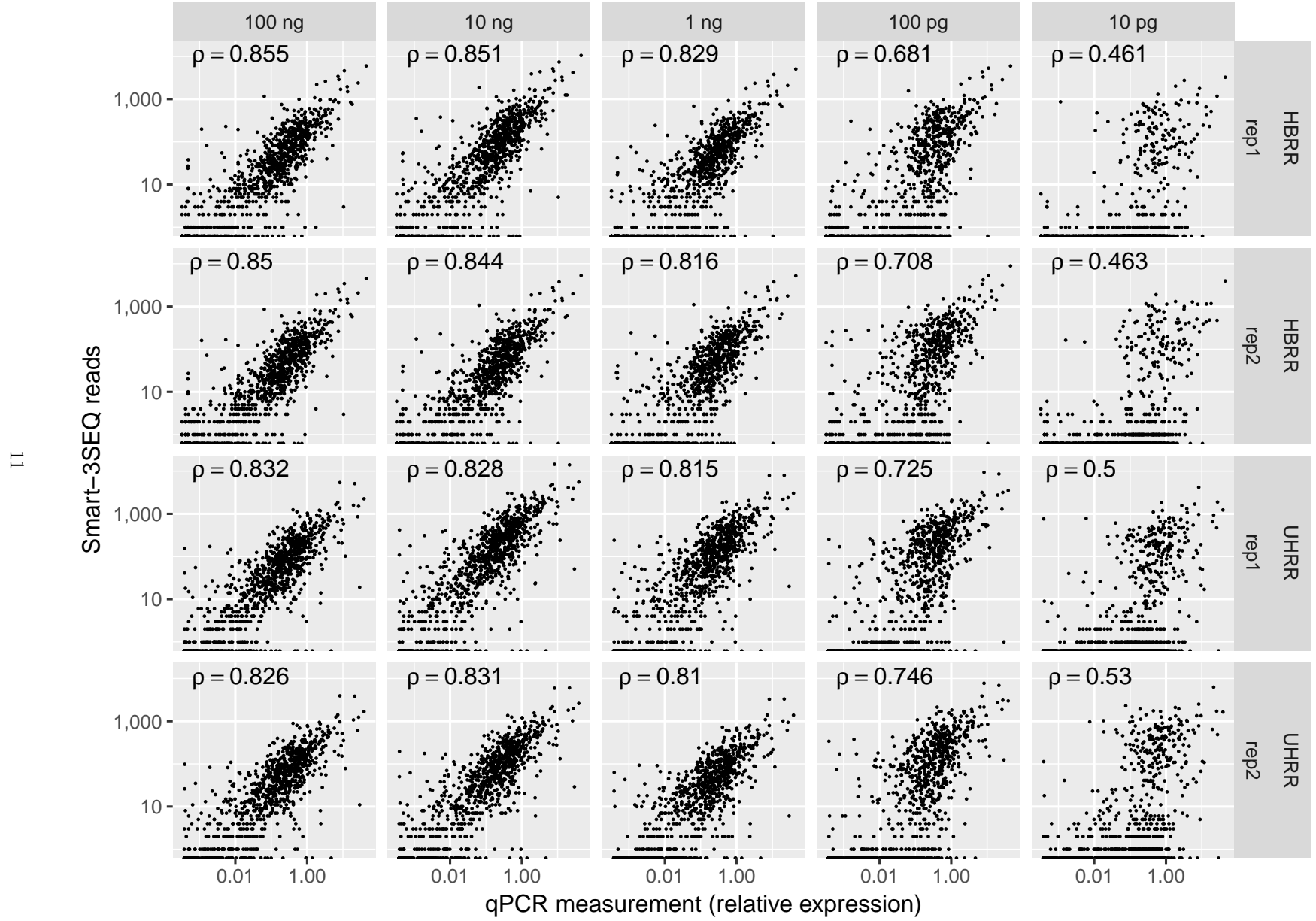
Figure S10: Correspondence of Smart-3SEQ results with TaqMan qPCR measurements. Each point is a single gene with available TaqMan qPCR data. \rho : Spearman's rank correlation.
