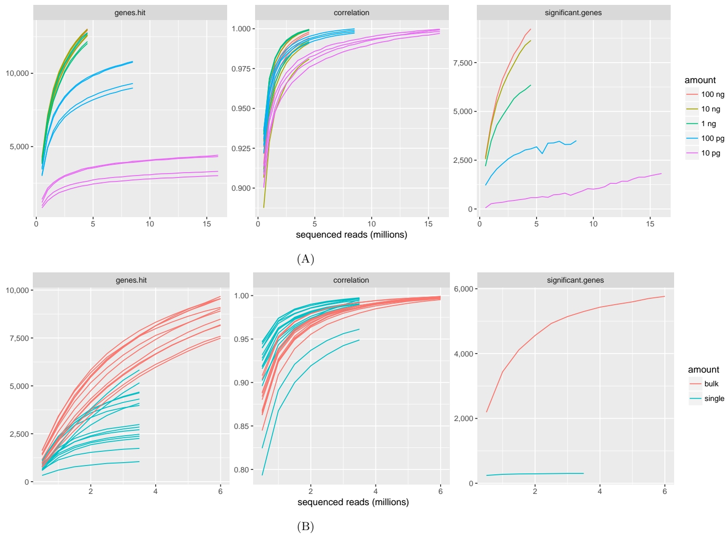
Figure S20: Diminishing returns from increased sequencing depth. Results are simulated by binomial subsampling of the gene-aligned read counts. genes.hit : number of genes with at least 10 reads aligned. correlation : Pearson correlation of gene expression values (as \log_{10}(c + 1) for read count c ) between subsampled data and original. significant.genes : number of genes with p_{\text{adjusted}} < 0.05 for significant differential expression between biological categories. A: Dilution series of human reference RNAs (HBR vs. UHR); 2 library replicates per condition at each dilution. B: Bulk tissue and single cells from LCM on FFPE tissue (macrophage vs. DCIS; single DCIS-labeled cells lacking ERBB2 amplification not included); 6 dissection replicates per condition for bulk and 10 vs. 5 single cells.
