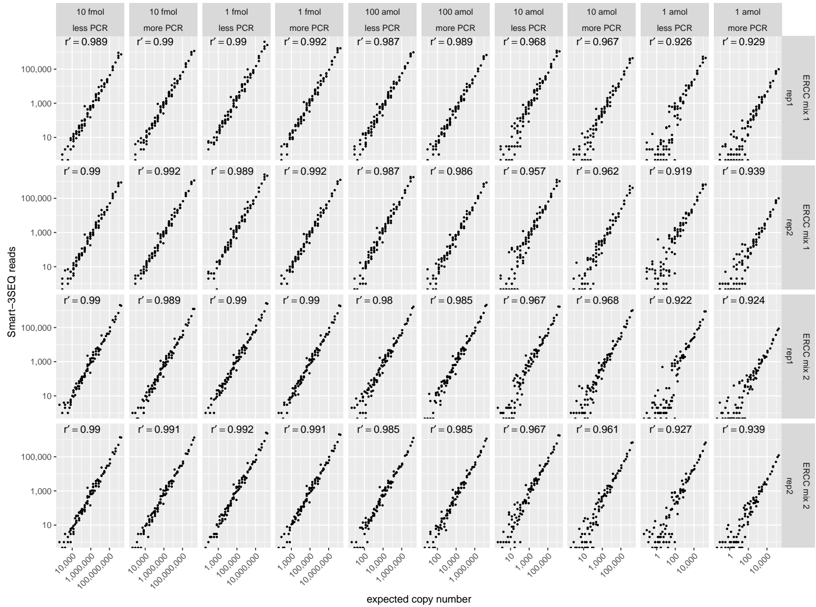
Figure S6: Accuracy of Smart-3SEQ. Standard curves from ERCC experiment. Each point is a single transcript.
