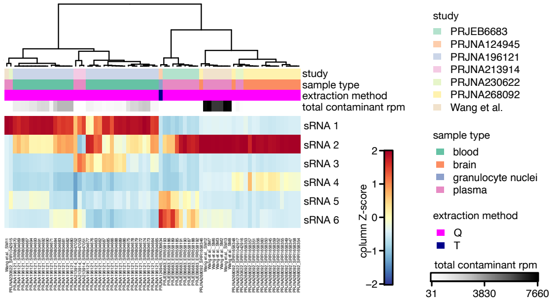
Supplementary Figure 2. Detection of contaminants in published datasets. Heatmap showing the relative abundances of the confirmed contaminant sequences in published sRNA sequencing data of low-biomass samples. Only samples for which any of the confirmed contaminants were detected are shown. Extraction methods: Q: regular QIAGEN miRNeasy; T: TRIZOL. rpm: reads per million.
