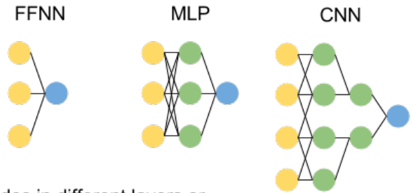
Figure 1: Neural networks come in many different forms. Left: a key for the various types of nodes used in neural networks. Simple FFNN: a feed forward neural network in which inputs are connected via some function to an output node and the model is trained to produce some output for a set of inputs. MLP: the multi-layer perceptron is a feed forward neural network in which there is at least one hidden layer between the input and output nodes. CNN: the convolutional neural network is a feed forward neural network in which the inputs are grouped spatially into hidden nodes. In the case of this example, each input node is only connected to hidden nodes alongside their neighboring input node. Autoencoder: a type of MLP in which the neural network is trained to produce an output that matches the input to the network. RNN: a deep recurrent neural network is used to allow the neural network to retain memory over time or sequential inputs. This figure was inspired by the Neural Network Zoo by Fjodor Van Veen.
