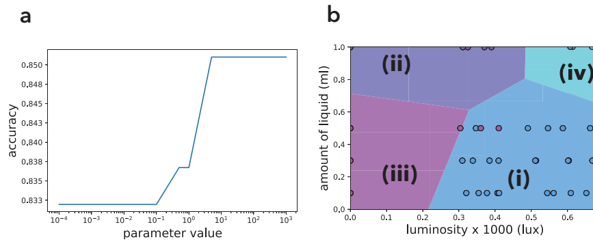
Figure S7: Experimental results. The parameter for LinearSVC is adjusted by a 10-fold cross-validation (a). The result of classification is shown in (b). Under light and dry conditions (i), only fruiting bodies are formed, and only macrocysts are formed under dark conditions with a large amount of culture liquid (ii). Both fruiting bodies and macrocysts are formed under dark conditions with less liquid (iii), and neither is formed under light conditions with excess culture liquid (iv).
