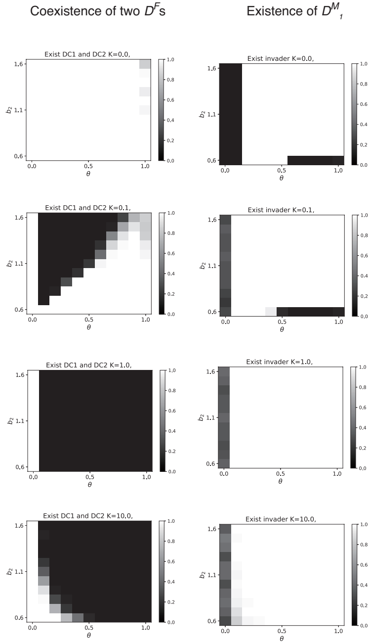
Figure S6: Invasion of D_1^M into the population where D^F s coexists in the agent-based model. The coexistence of D_1^F and D_2^F is an evolutionarily stable state if the defection of macrocyst formation does not occur. However, coexistence collapses due to the invasion of defectors of macrocyst formation D_1^M under weak selection ( K = 1, 10 , left column). On the other hand, the invader D_1^M can be maintained at a frequency greater than 0.01 regardless of the strength of selection under a wide range of parameter values b_2 and \theta (right column). The other parameters are \epsilon_1 = 10^{-5} , a_2 = 0.5 , \epsilon_2 = 10^{[-5]} , h = 0.5 , and \epsilon_0 = 10^{-6} .
