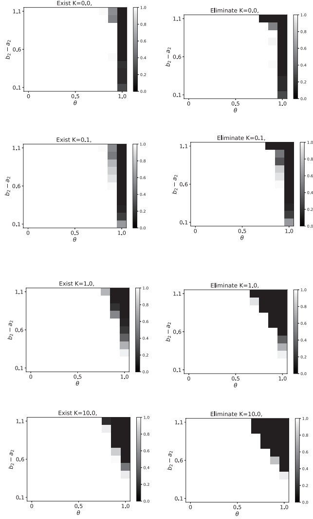
Figure S4: Invasion of C_1 to D^M in the population in the agent-based model. Regardless of the strength of the selection, the cooperator C_1 can invade (left) and exclude (right) the same mating type defector of macrocyst formation D_1^M and the counterpart of the other mating type D_2^M unless \theta is large. The other parameters are a_1 = 1 , a_2 = 0.5 , \epsilon_2 = 10^{-5} , h = 0.5 , and \epsilon_0 = 10^{-6} .
