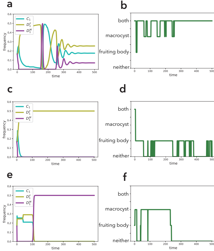
Figure S8: Evolutionary dynamics under a dynamic environment. By introducing a changing environment, we relaxed the assumption that fruiting bodies coexist with macrocysts. In the initial condition, all six strategies coexist at the same frequencies. In the evolutionary dynamics, only the dynamics of mating type 1 are shown because the evolutionary dynamics are symmetric among mating types. Based on the environment, all strategies perform (i) only fruiting body formation, (ii) only macrocyst formation, (iii) both fruiting body formation and macrocyst formation, or (iv) neither fruiting body formation nor macrocyst formation. Three examples of the discrete replicator dynamics are shown in (a), (c), and (e) under environmental dynamics (b), (d), and (f), respectively. The environmental dynamics affect the results of the evolutionary dynamics. The parameters are a_1 = 1 , b_1 = 1.2 , \epsilon_1 = 10^{-4} , a_2 = 0.6 , b_2 = 1.2 , \epsilon_2 = 10^{-4} , h = 0.5 , \epsilon_0 = 10^{-6} , and \sigma = 0.05 . See SI text for the detail of the simulation.
