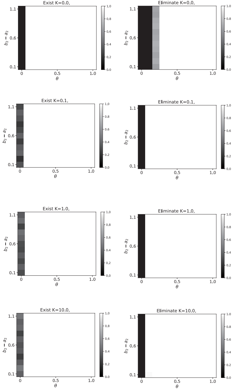
Figure S5: Invasion of D_1^M to D^F in the population in the agent-based model. Regardless of the strength of the selection, D_1^M cannot invade the same mating type defector of fruiting body formation D_1^F , but it can invade the other mating type ones D_2^F . Unless selection is very strong ( K = 0.1, 1, 10 ), D_1^M can exclude the other mating type defector of fruiting body formation. If K = 0 , this exclusion occurs if \theta \geq 0.3 . The other parameters are \epsilon_1 = 10^{-5} , a_2 = 0.5 , \epsilon_2 = 10^{-5} , h = 0.5 , and \epsilon_0 = 10^{-6} .
