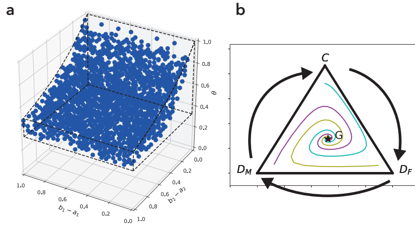
Figure S1: Discrete replicator dynamics without mating types. In the discrete replicator dynamics, the interior equilibrium is not always stable if the payoff matrix represents the RSP game. The conditions where the interior equilibrium is stable in the discrete replicator dynamics are shown as blue dots, whereas those from the continuous replicator dynamics are inside the black dashed lines in (a). The parameters in (a) are a_1 = 1 , \epsilon_1 = 10^{-4} , a_2 = 0.5 , \epsilon_2 = 10^{-4} , \theta = 0.5 , h = 0.5 , and \epsilon_0 = 10^{-6} . The examples of the discrete replicator dynamics that converge to the interior equilibrium G are shown in (b). The parameters in (b) are a_1 = 1 , b_1 = 1.5 , \epsilon_1 = 10^{-4} , a_2 = 0.5 , b_2 = 1.2 , \epsilon_2 = 10^{-4} , \theta = 0.5 , h = 0.5 , and \epsilon_0 = 10^{-6} .
