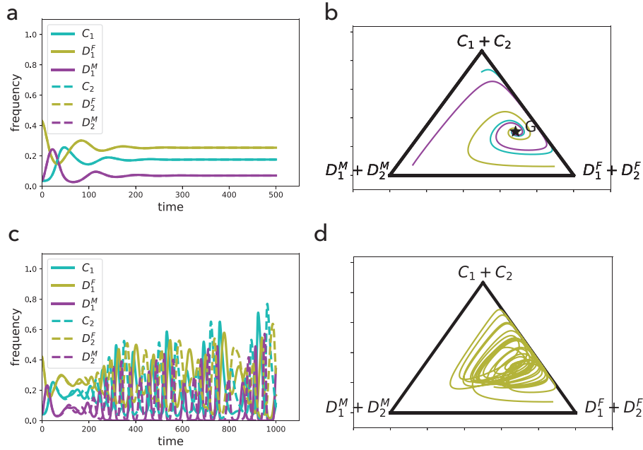
Figure S2: Continuous replicator dynamics that include mating types. In these examples, there exists six strategies, and the initial sex ratio has a large effect on evolutionary dynamics. When the initial sex ratio is equal and the initial condition is symmetric over the mating types, the dynamics converge to the stable point (a), and this holds when the initial condition is changed (b). If the initial sex ratio is not equal (in this case C_1 : D_1^F : D_1^M : C_2 : D_2^F : D_2^M = 1 : 10.1 : 1 : 1 : 10 : 1 ), the dynamics never converge to the stable point (c). The dynamics in the phase space is shown in (d). Note that the cooperators C_1 and C_2 are not excluded even though the dynamics do not converge to the stable point. The parameters are a_1 = 1 , b_1 = 1.2 , \epsilon = 10^{-4} , a_2 = 0.6 , b_2 = 1.2 , \epsilon_2 = 10^{-4} , \theta = 0.9 , h = 0.5 , and \epsilon_0 = 10^{-6} .
