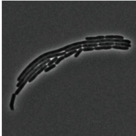
\Delta lon
