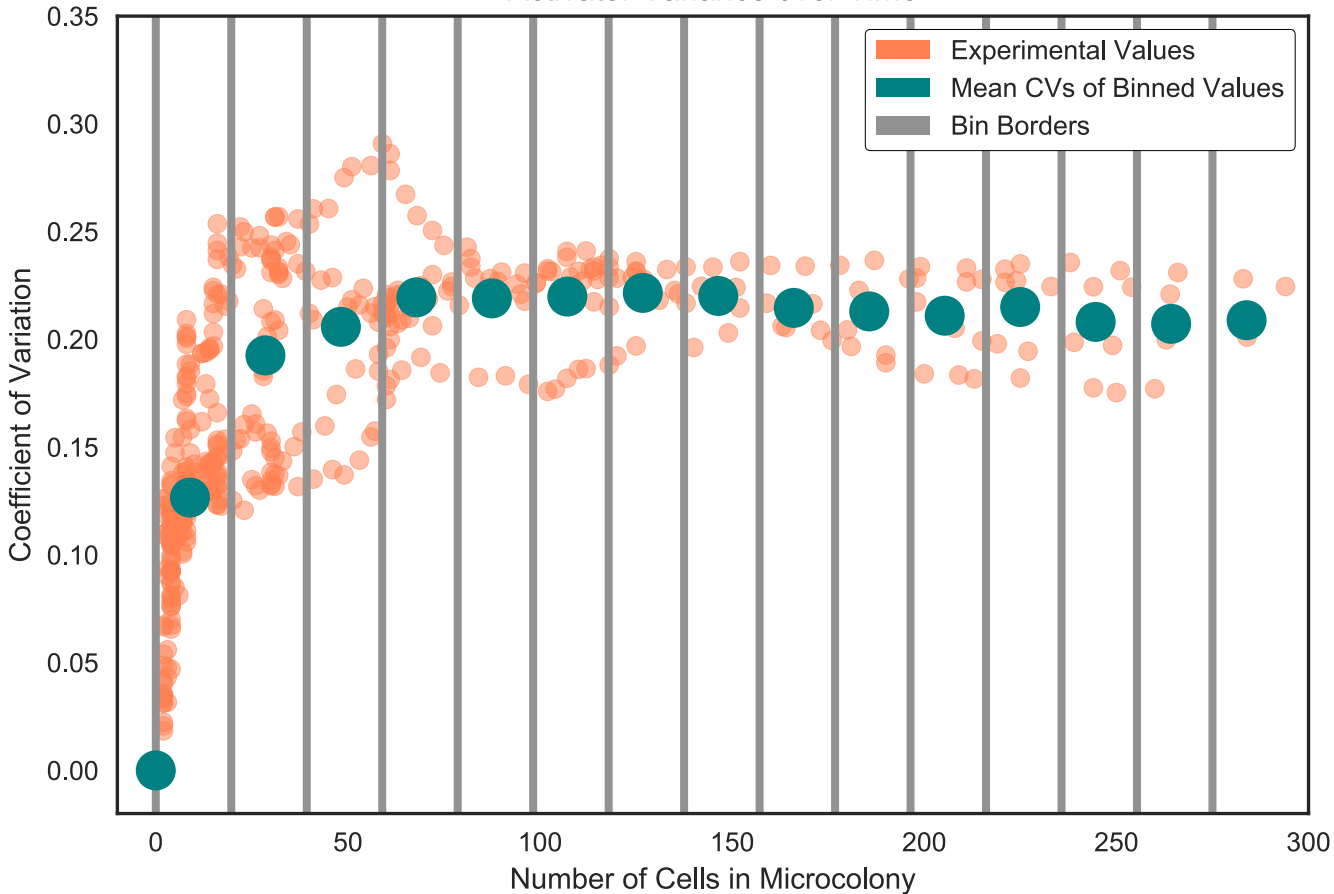
Activator Variance over Time
