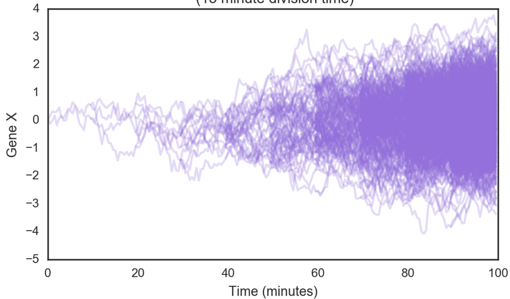
Stochastic Trajectories with Cell Division (15 minute division time)
