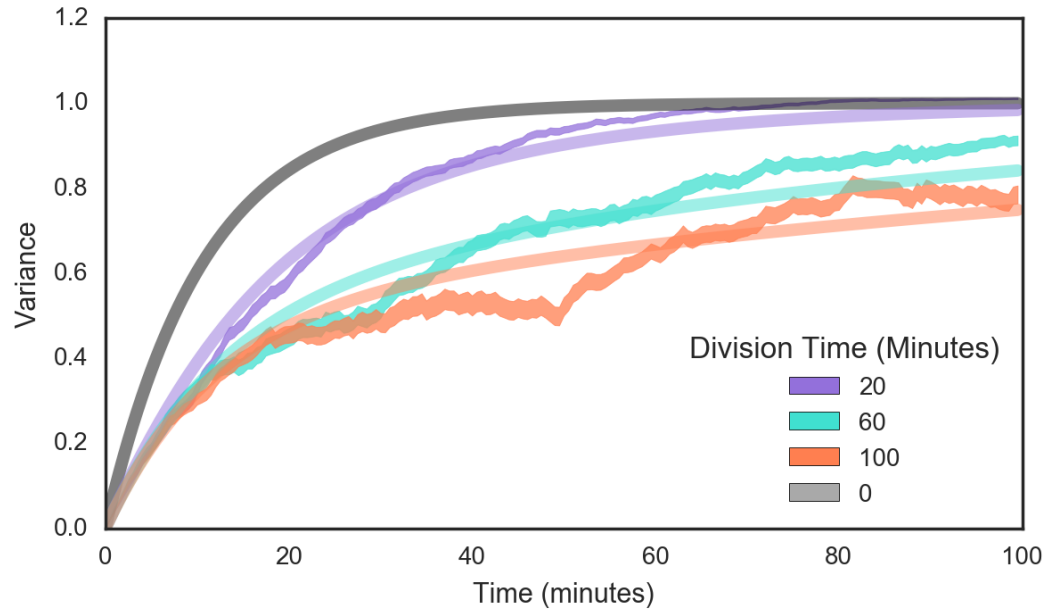
Variance over Time as a Function of Growth Rate
