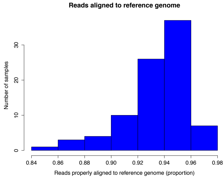
S1 Fig. Histogram of the proportion of reads passing quality filter that aligned to the references genome.
