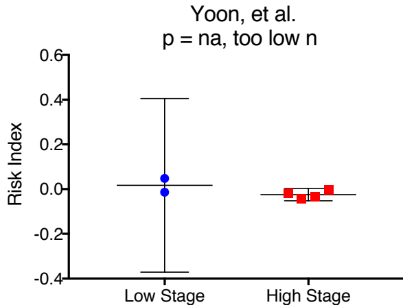
S3 Fig. Column dot plots of the risk indices determined using the stage-relevant model generated in this work to the microbiome data from Flemer, et al. (left) and Yoon, et al. (right).
