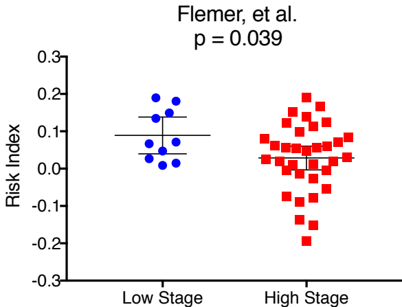
S3 Fig. Column dot plots of the risk indices determined using the stage-relevant model generated in this work to the microbiome data from Flemer, et al. (left) and Yoon, et al. (right).
