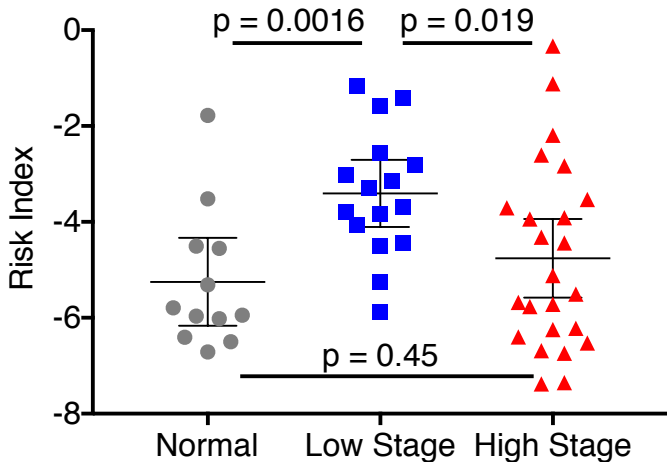
S4 Fig. Column dot plots of the risk indices calculated using a new model designed to separate microbial communities from normal, low stage, and high stage tumors. Normals included in this model and figure are from healthy individuals from an independent study, not from patient matched samples.
