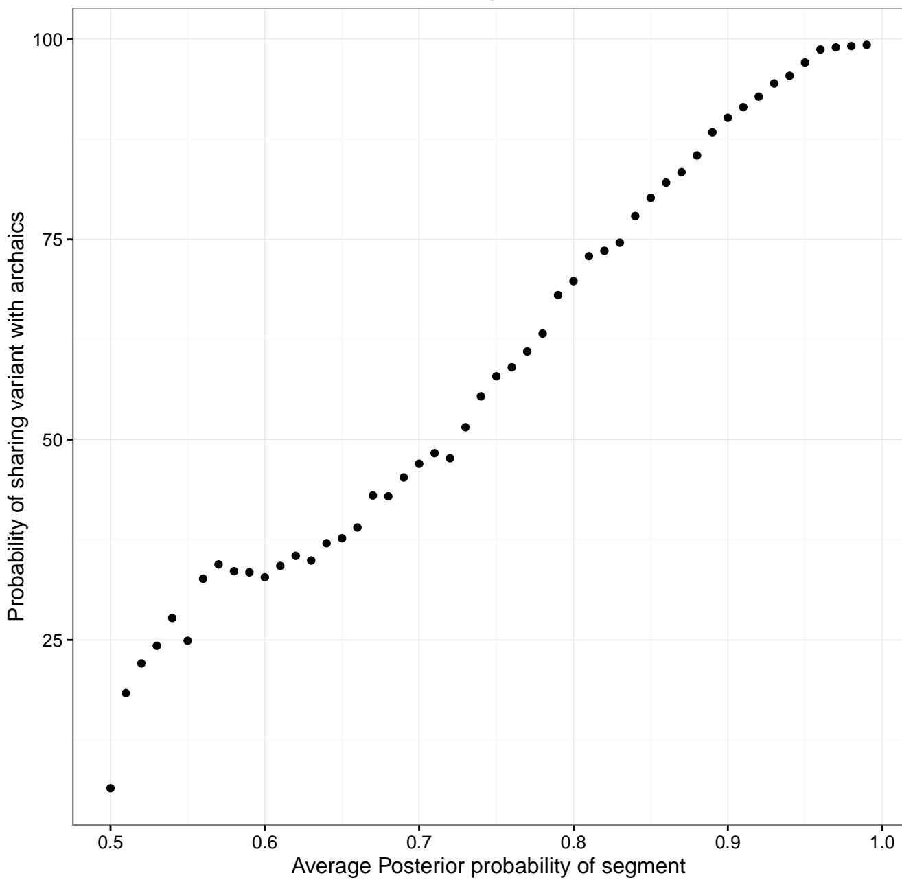
Probability of sequence sharing variant with archaic hominins
