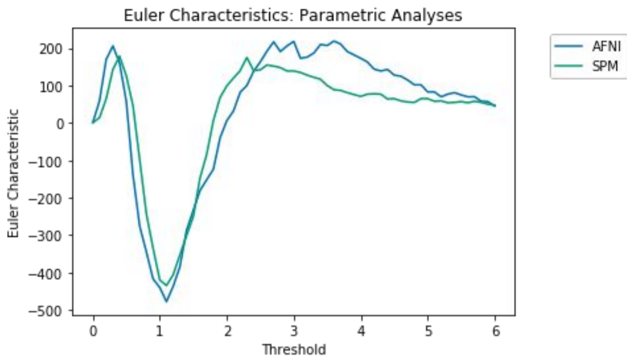
Figure S12. ds000120 Inter-Software Comparison, Euler Characteristic Curves for F-Statistic Maps
