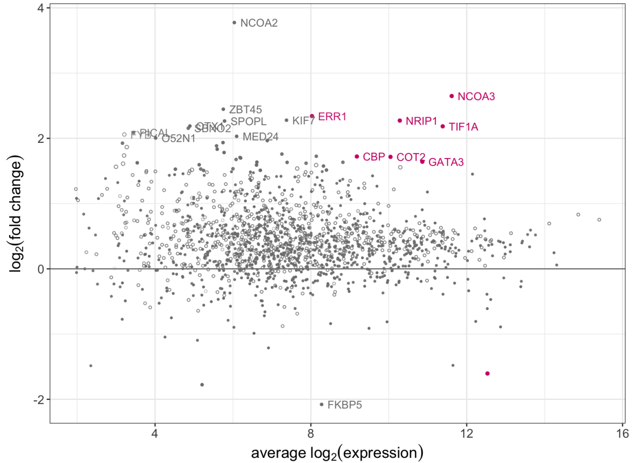
Figure 48: MA plot of the average intensity against log 2 fold change for the ER 45min vs ER 0min comparison (excluding peptides with missing intensities, no normalization). Top ranking differentially-expressed proteins with false discovery rate below 0.05 are highlighted in pink. Open circles indicate that the protein is non-specific from the IgG control comparison.
