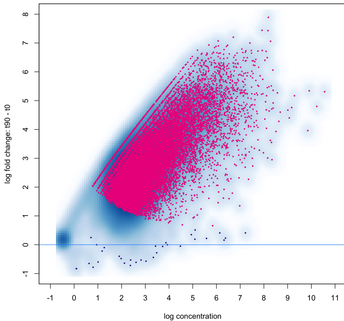
Figure 8: MA plot for Contrast 90mins vs 00mins, highlighting each individual peak. Significant peaks are highlighted in red
