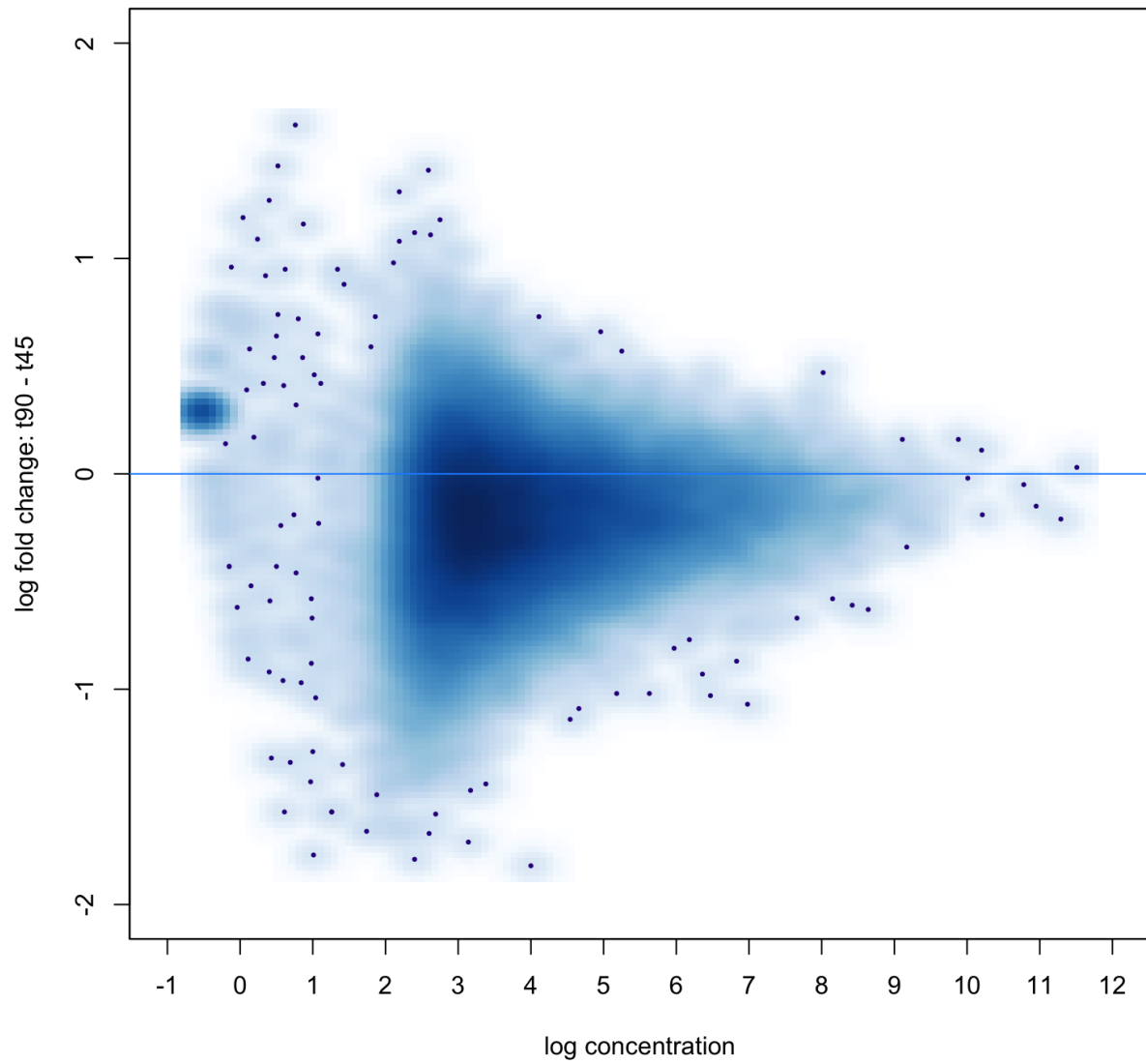
Figure 7: MA plot for Contrast 90mins vs 45mins, highlighting each individual peak. Significant peaks are highlighted in red
