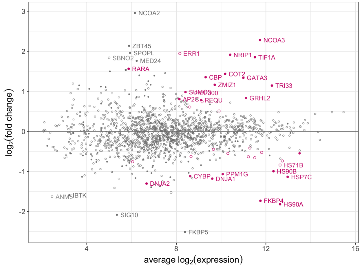
Figure 52: MA plot of the average intensity against log 2 fold change for the ER 45min vs ER 0min comparison (excluding peptides with missing intensities, quantile normalization). Top ranking differentially-expressed proteins with false discovery rate below 0.05 are highlighted in pink. Open circles indicate that the protein is non-specific from the IgG control comparison.
