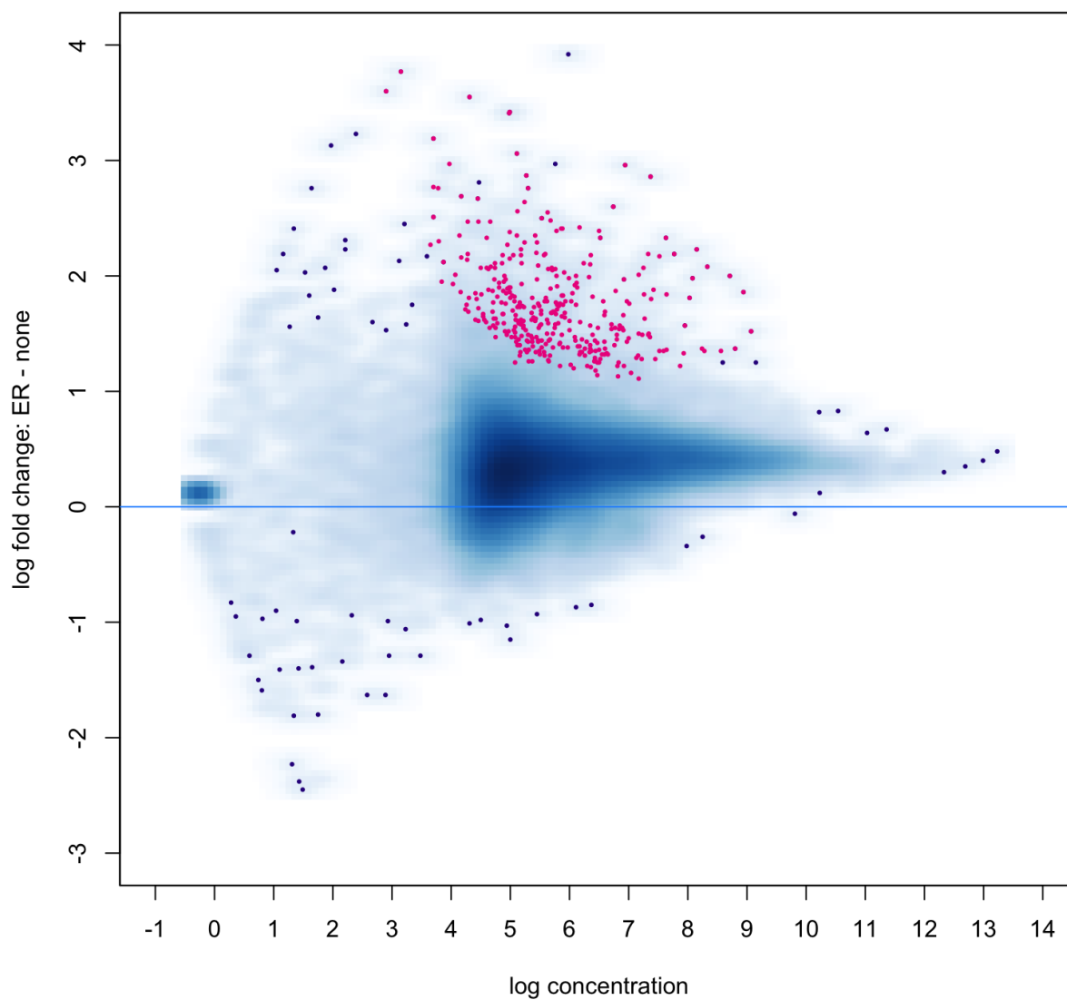
Figure 83: MA plot showing changes in GRHL2 binding before and after treatment with 100nM E2.
