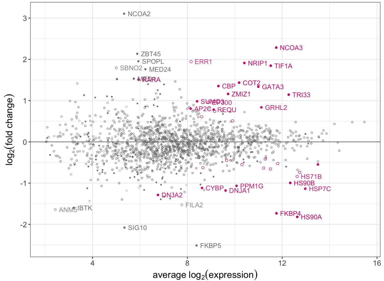
Figure 68: MA plot of the average intensity against log 2 fold change for the ER 45min vs ER 0min comparison (KNN nearest neighbour averaging imputation of missing values, quantile normalization). Top ranking differentially-expressed proteins with false discovery rate below 0.05 are highlighted in pink. Open circles indicate that the protein is non-specific from the IgG control comparison.
