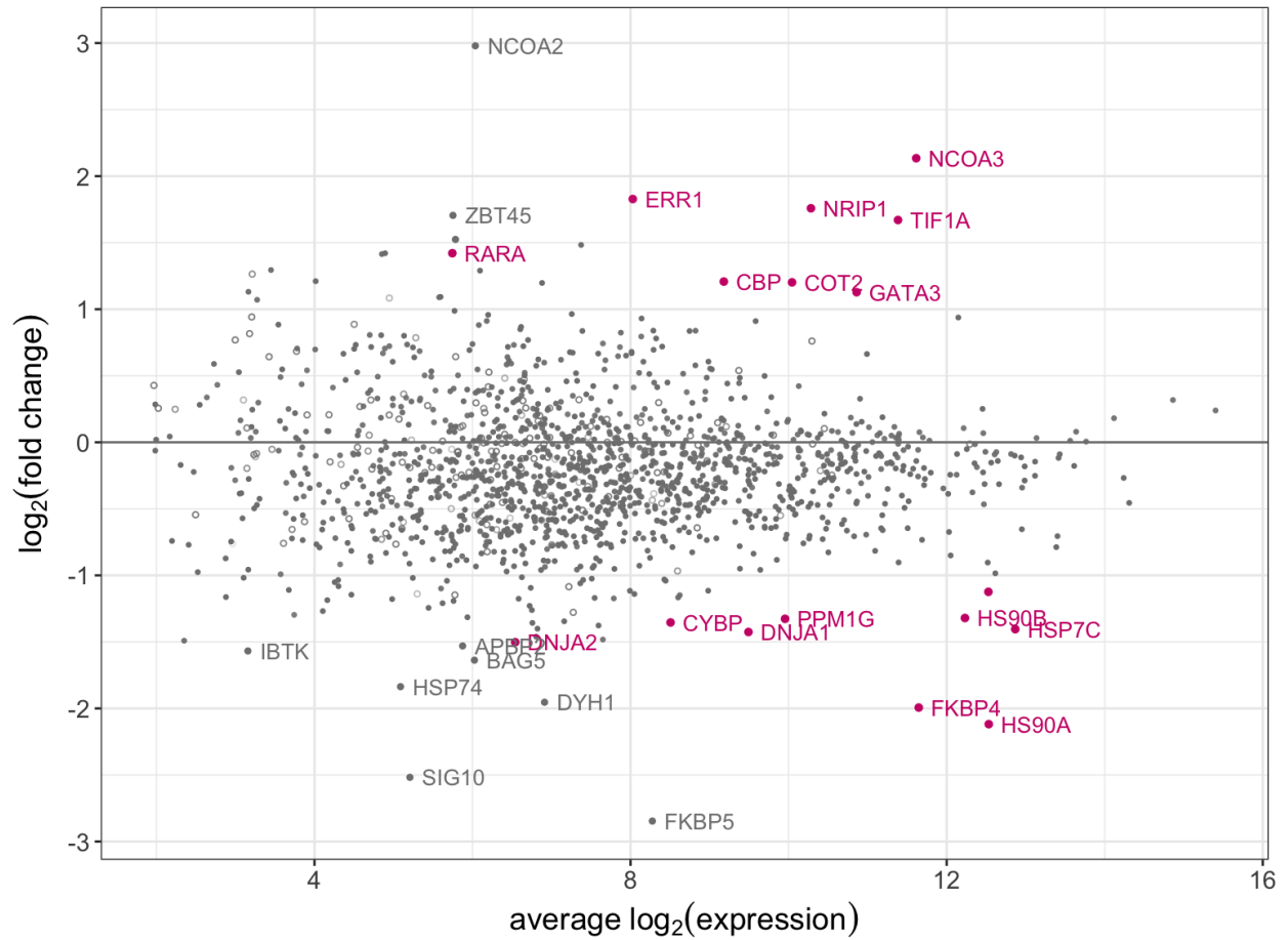
Figure 64: MA plot of the average intensity against log 2 fold change for the ER 45min vs ER 0min comparison (excluding peptides with missing intensities, scale normalization using top 10 IgG peptides). Top ranking differentially-expressed proteins with false discovery rate below 0.05 are highlighted in pink. Open circles indicate that the protein is non-specific from the IgG control comparison.
