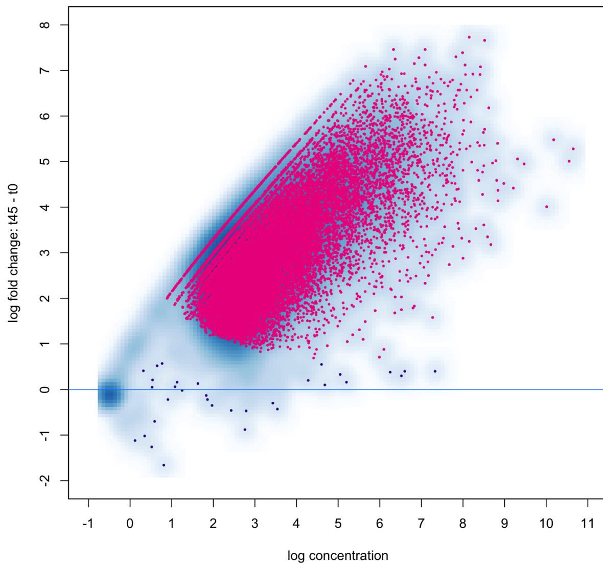
Figure 9: MA plot for Contrast 45mins vs 00mins, highlighting each individual peak. Significant peaks are highlighted in red
