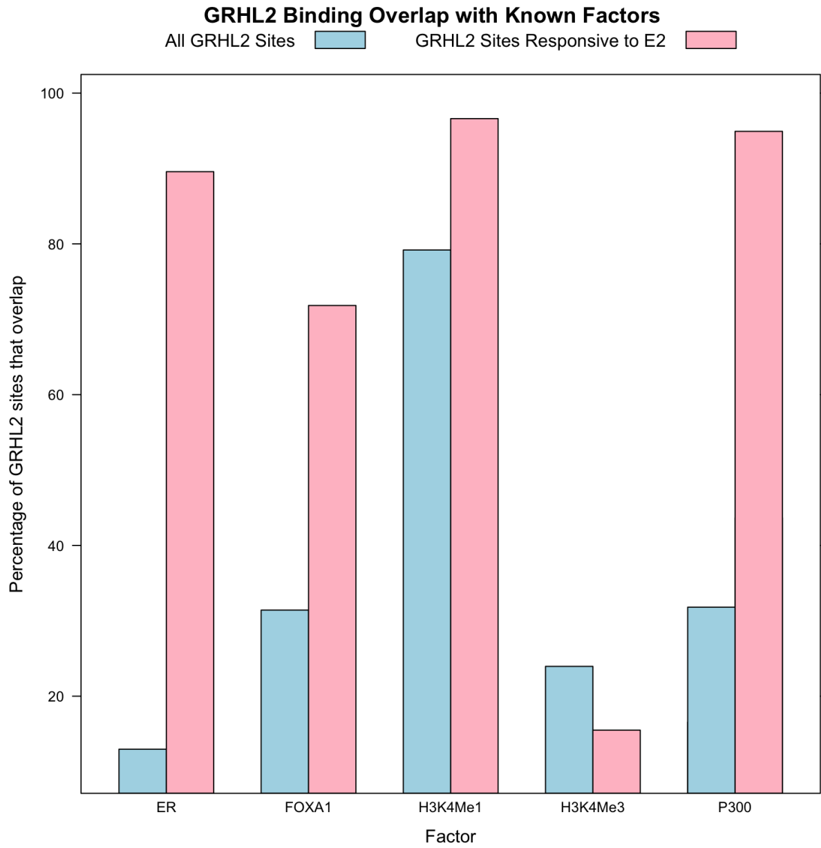
Figure 88: GRHL2 binding overlap with known factors
