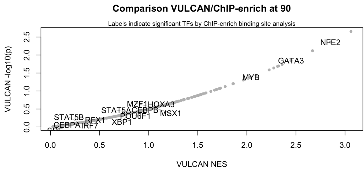
Figure 39: Comparison of results from the VULCAN and ChIP-enrich methods
