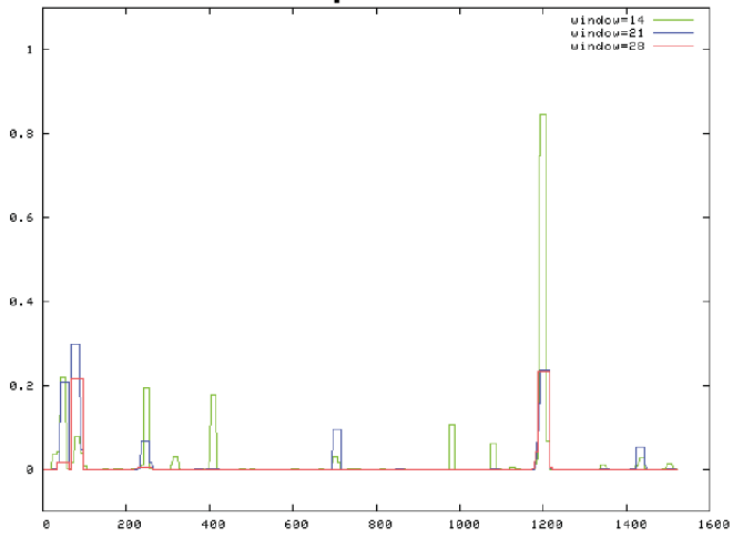
Yr5 protein without BED domain
