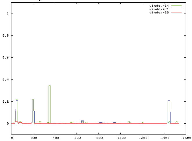
Yr7 protein without BED domain
