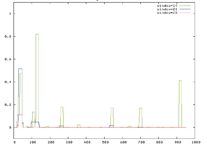
Pm3 protein
