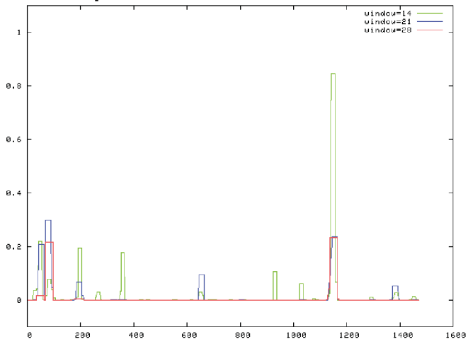
Yr7 protein
