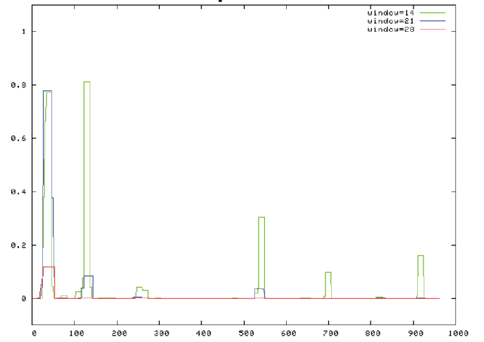
Mla10 protein
