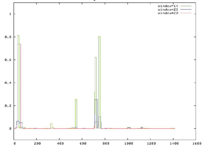
RPS5 protein
